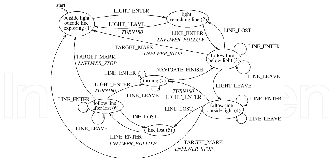
Figure17. Example of a manually designed FSA coordination for the line-follower module
