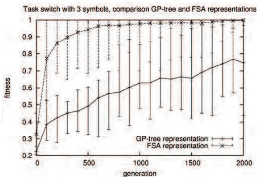
Figure 7. Average of the best fitness from 15 (GP) or 34 (FSA) runs of the switch task with three symbols, tournament selection, and other parameters as in the four-symbol experiment. The final fitness of all FSA runs outperforms the final fitness of the best GP-tree run
