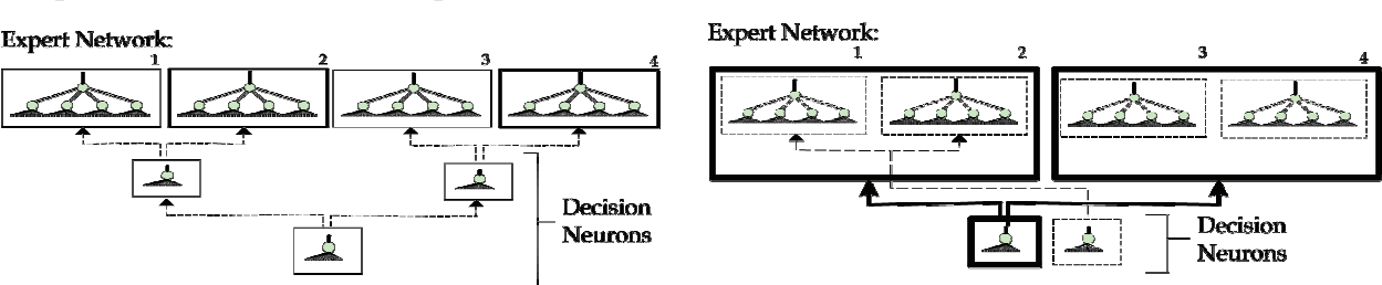
Figure 7. (Left) BDT Architecture with 4 expert networks and 3 decision neurons. (Right) BRL Architecture with 4 expert networks and 2 decision neurons
