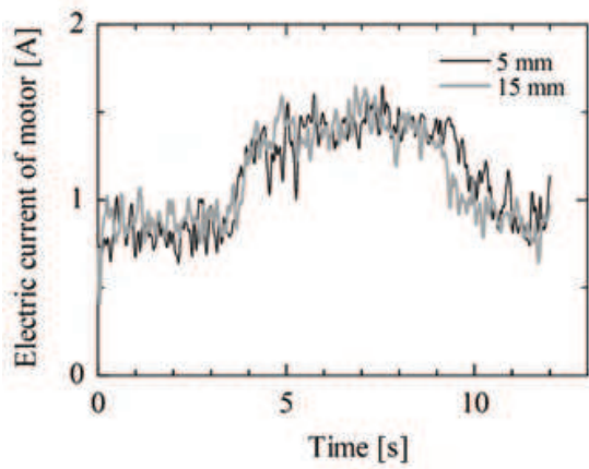
(a) Time response of the electric current of motor
