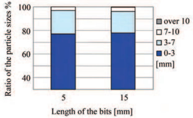
(b) Relationship between length of the bits and ratio of the particle sizes
