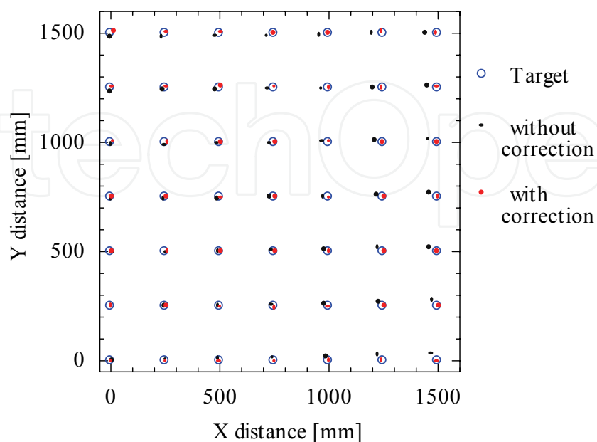
Fig. 16. Result of the position measurement
