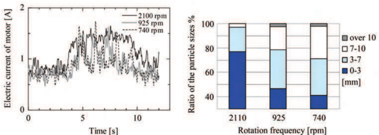
(a) Time response of the electric current of motor
