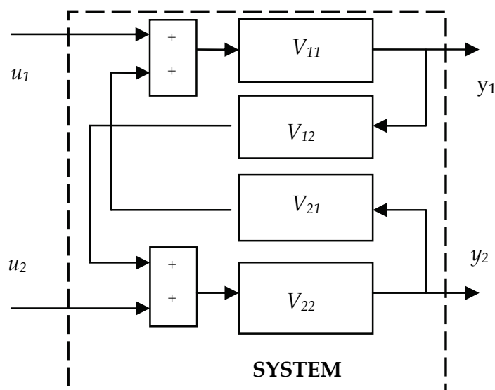
Fig. 6. The exemplary V-structure for 2 inputs and 2 outputs.
