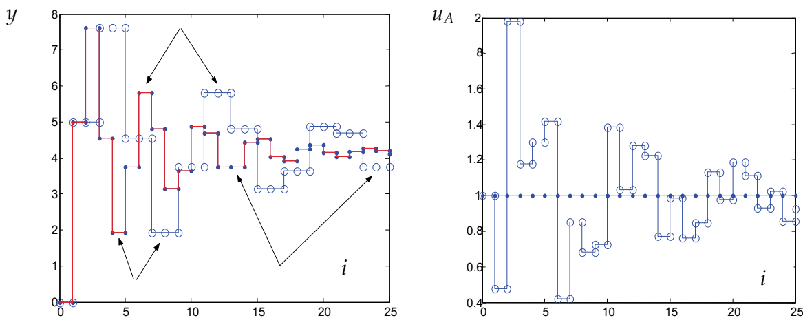
Fig. 3. Left position: the reference response of system (6) to signal u(i) = 1(i) – curve distinguished by "." – and response of system (6) obtained as output signal of structure in Fig. 2 – curve distinguished by "o". Note, that consecutive amplitudes of both responses are identical (compare chosen referring amplitudes indicated by arrows). Right position: reference input signal u(i) = 1(i) and input signal u_A(i) of system (6) when included to structure in Fig. 2 as SYSTEM.
