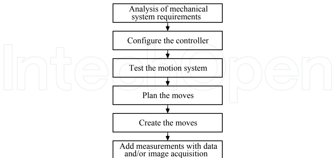
Fig. 13. Generic steps for designing a motion application.
