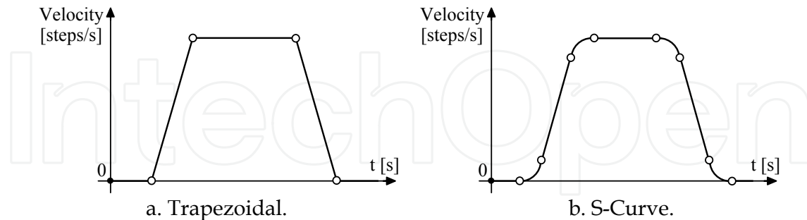
Fig. 5. Move Profile.
