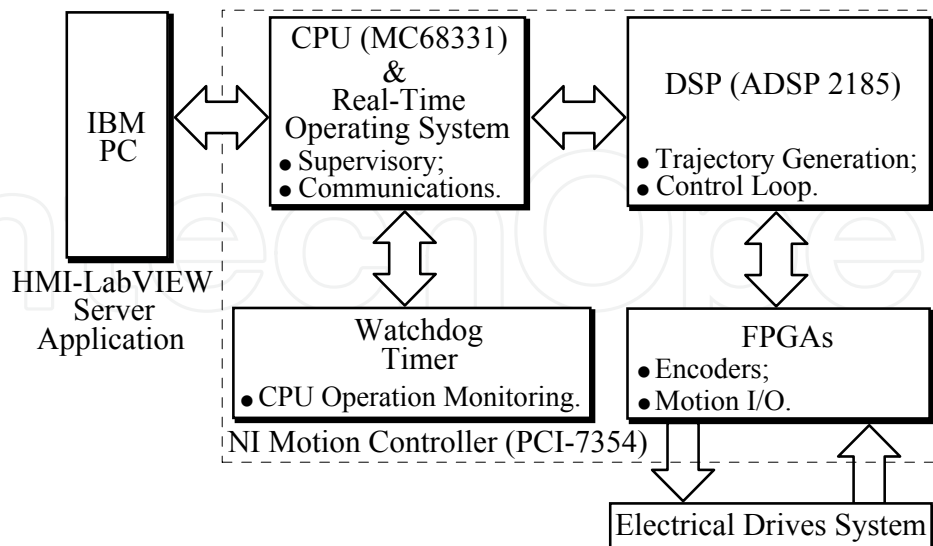
Fig. 3. Motion controller board structure.
