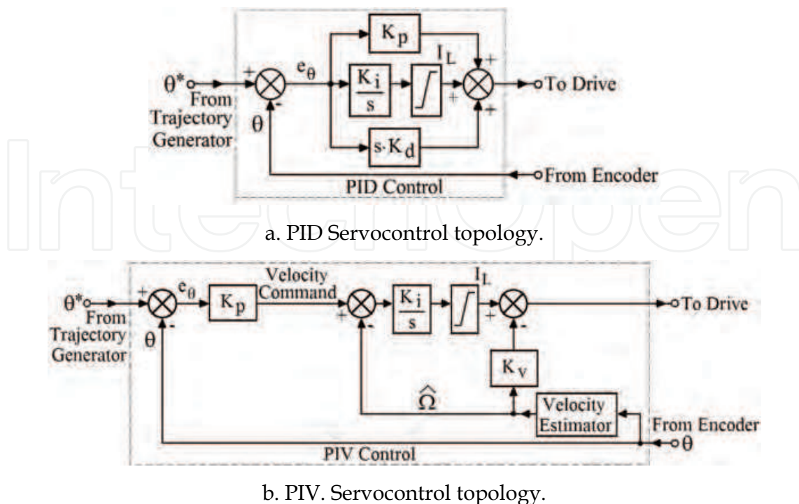
Fig. 11. Servocontrol topology.
