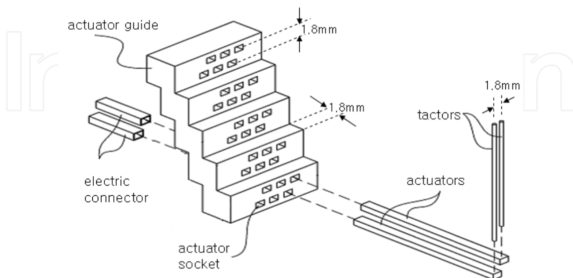
Fig. 1. Profile of the tactile display
