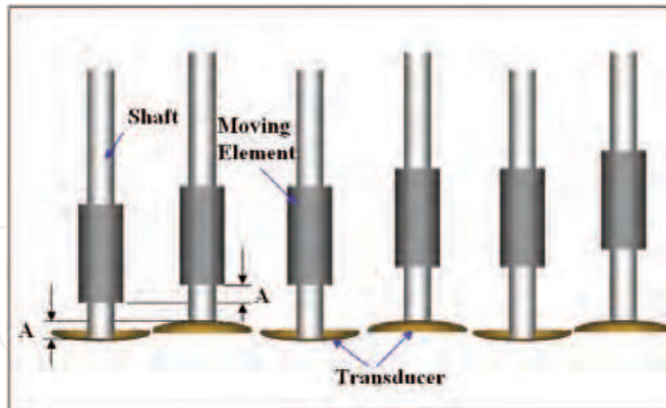
Fig. 7. Operation principle of an actuator
