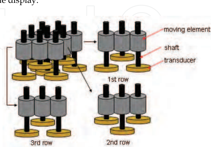
Fig. 8. Design drawing of a tactile display module
