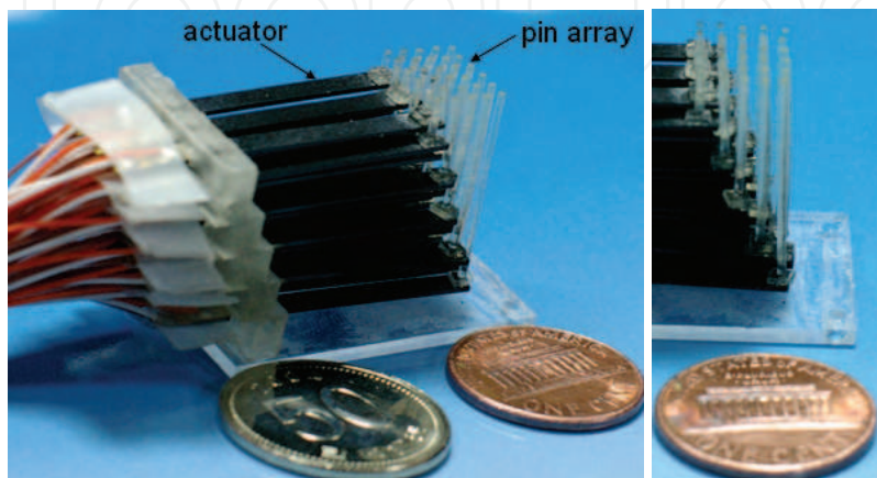
Fig. 2. The texture display unit
