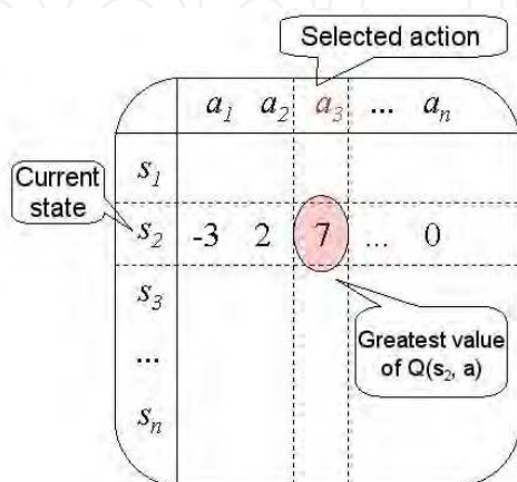
Fig. 2. Learning elements in a Q-Table
