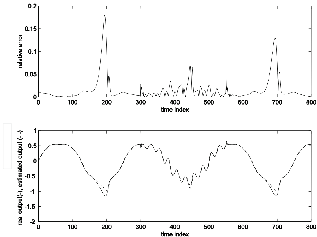
Fig. 3. Fuzzy identification using RL-based tuning algorithm and DAFM with initial conditions on [0.5, 1.5] .
