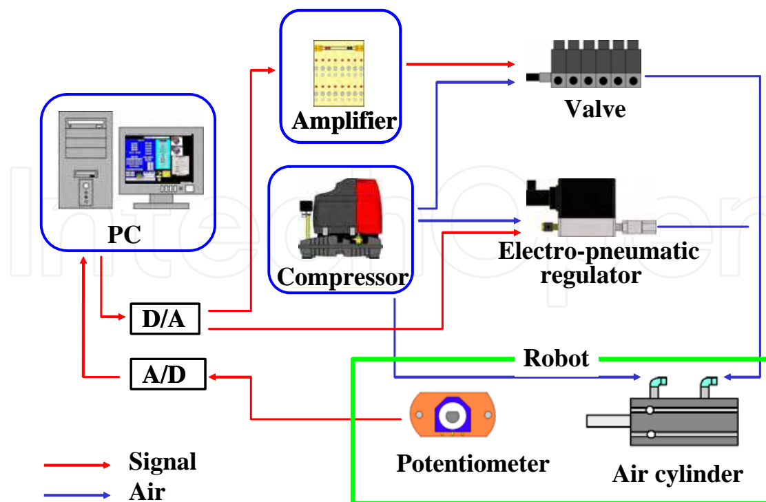
Figure 4. Control System
