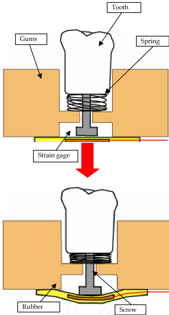
Figure 10. Mechanism of tooth sensor
