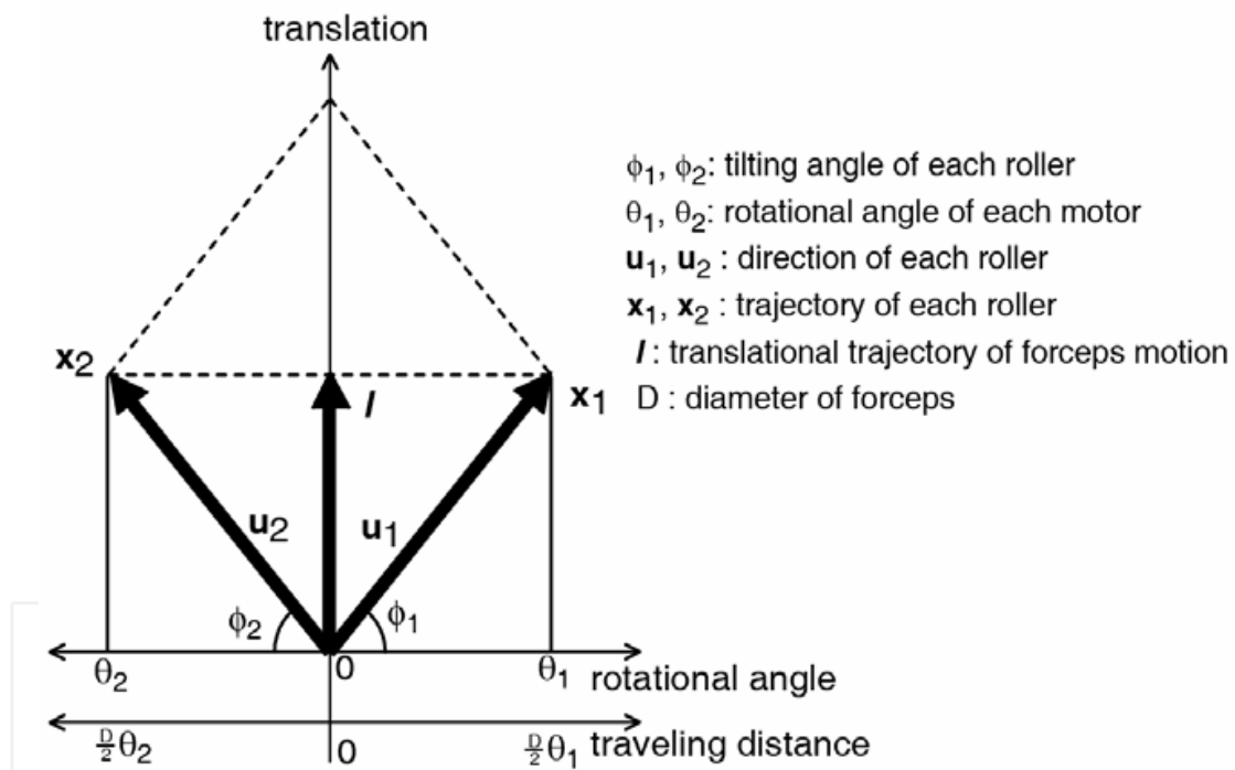
Figure 6. Translational motion can be shown by expanding the surface of forceps to a plane. Here, each roller has tilting angle of \phi_1 and \phi_2 . When outer cases are rotated by \theta_1 and \theta_2 , trajectory of each roller is as follows;
