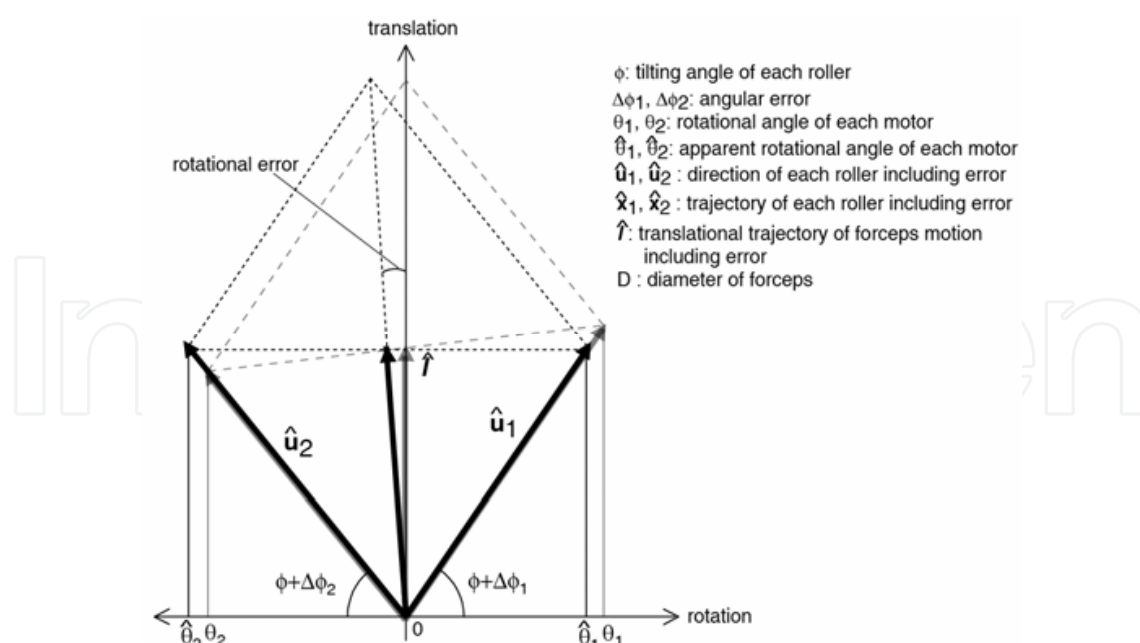
Figure 7. Error analysis of rotational error in translational motion
