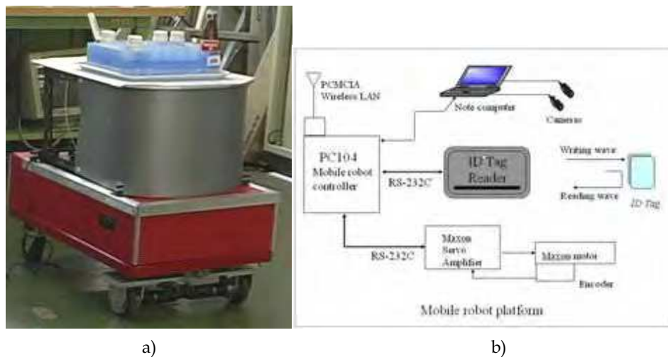
Figure 2. Mobile robot; (a) is the developed mobile; (b) is the structure of mobile robot platform
