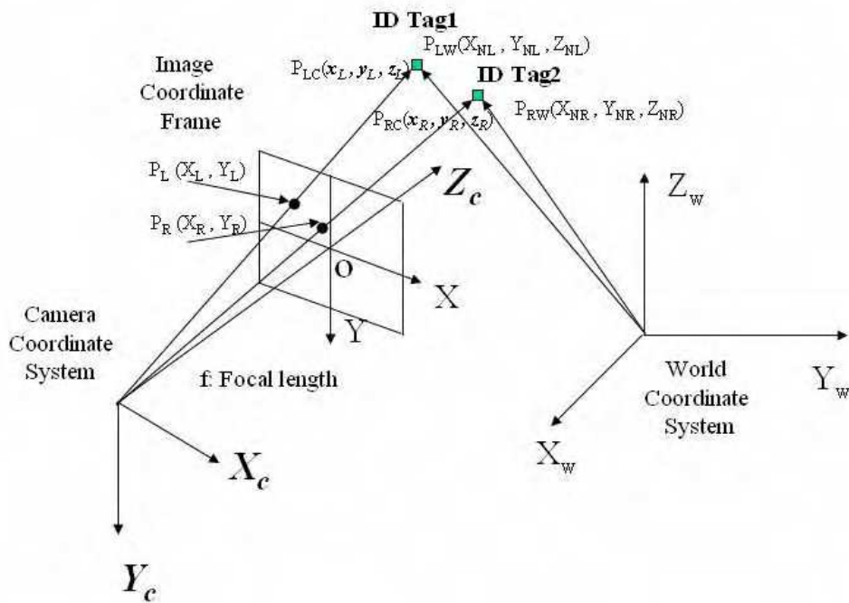
Figure 5. World coordinate system, camera coordinate system and image coordinate frame Figure 5 illustrates the relationship among World Coordinate System, Camera Coordinates System and Image Coordinates Frame used in our system. The origin of World Coordinate System was set at the corner of environment the mobile robot moves in. The origin of Camera Coordinates System was set at the focus of CCD camera mounted on the mobile robot. P_{LW}(X_{NL}, Y_{NL}, Z_{NL}) and P_{RW}(X_{NR}, Y_{NR}, Z_{NR}) are the coordinates of two ID tags in World Coordinate System. P_{LC}(x_L, y_L, z_L) and P_{RC}(x_R, y_R, z_R) are the coordinates of two ID tags in Camera Coordinate System. P_L(X_L, Y_L) and P_R(X_R, Y_R) are the projected coordinates of two ID tags in Image Coordinates Frame. According to coordinate transformation, we can calculate x_L, y_L, x_R, y_R and X_L, Y_L, X_R, Y_R . \theta is the orientation angle of the mobile robot in the world coordinate frame. x_r, y_r are the position of mobile robot relative to the node, which can be got by recognition with camera. Using these variables, the coordinates of camera (the coordinates of mobile robot X_m, Y_m in World Coordinate System can be calculated by equation (equation (6)).
