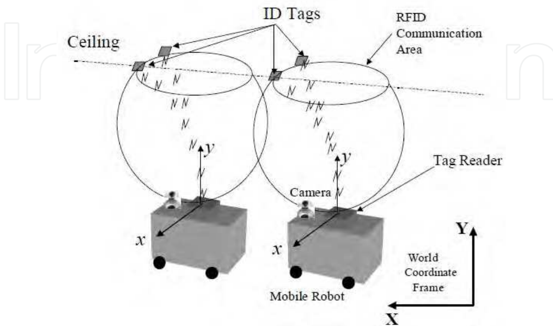
Figure 3. The principle of localization of mobile robot with RFID and camera
