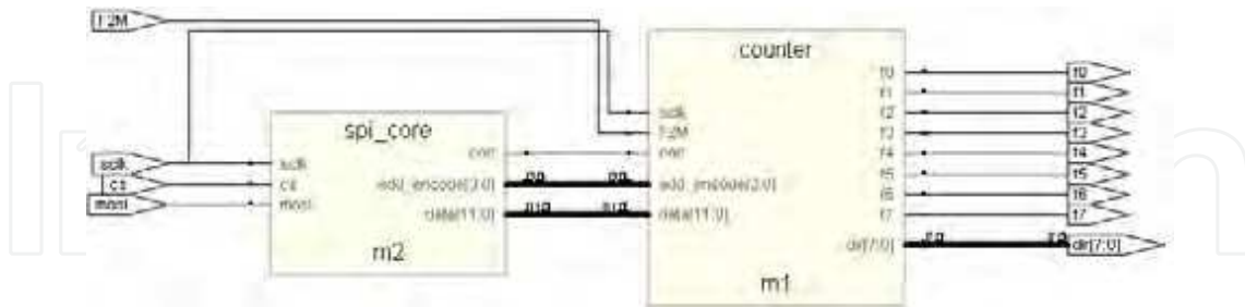
Fig. 15. Modules of the motor control system.
