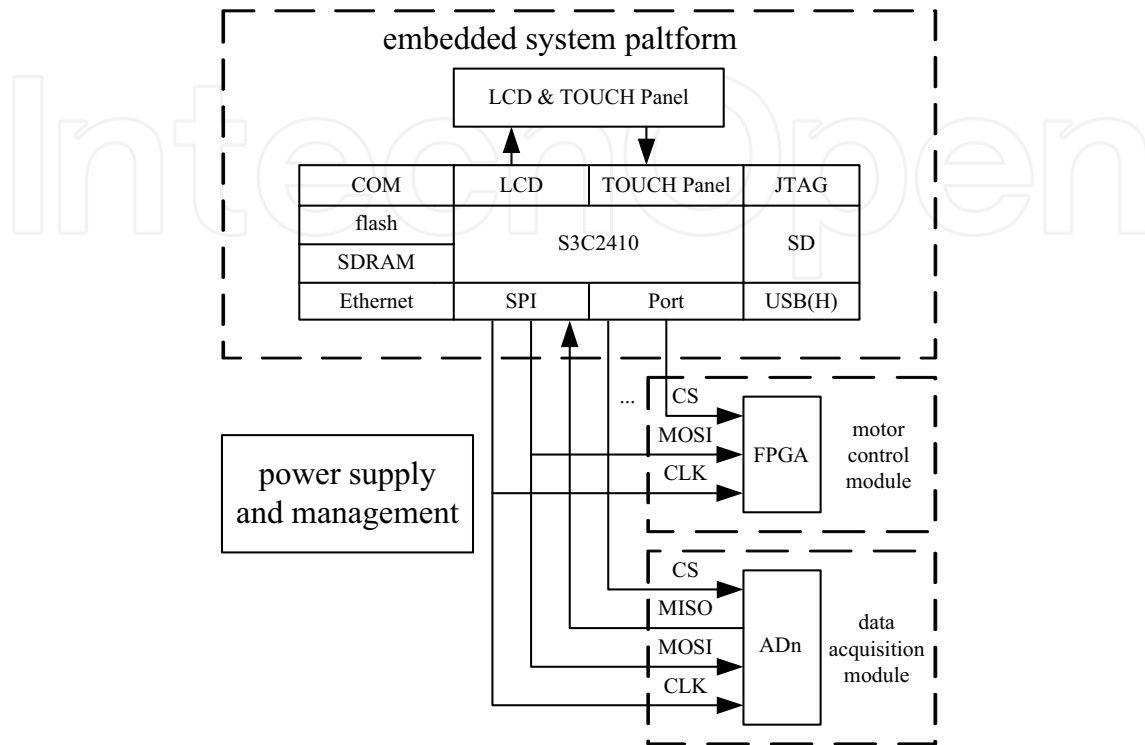
Fig.10. Functional partition of the embedded hardware platform.
