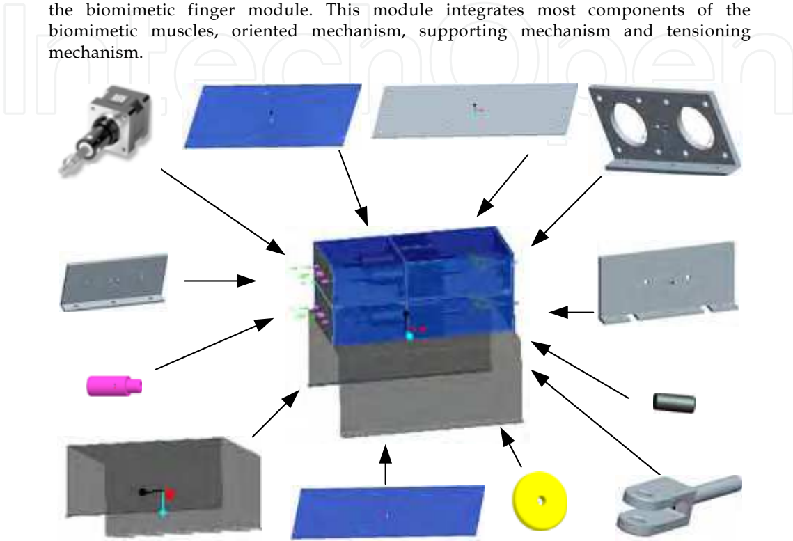
Fig. 4. Biomimetic muscle module.
