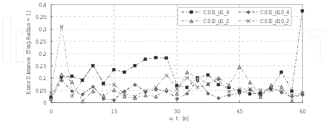
Fig. 7. The variance of error distances in time series. The first and second CSCI subject's data are presented as CSI1 and CSI2, accordingly. The 1 st day's data is shown as d1 and 10 th day's data as d10. The data are all last trials of the day.
