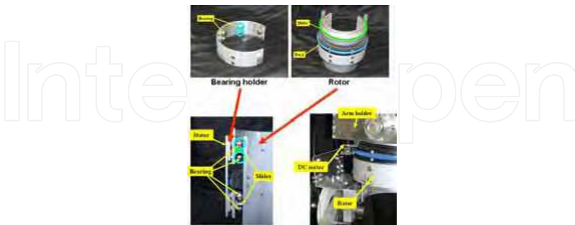
Fig. 2 Mechanism for shoulder inner/outer rotation motion assist.
