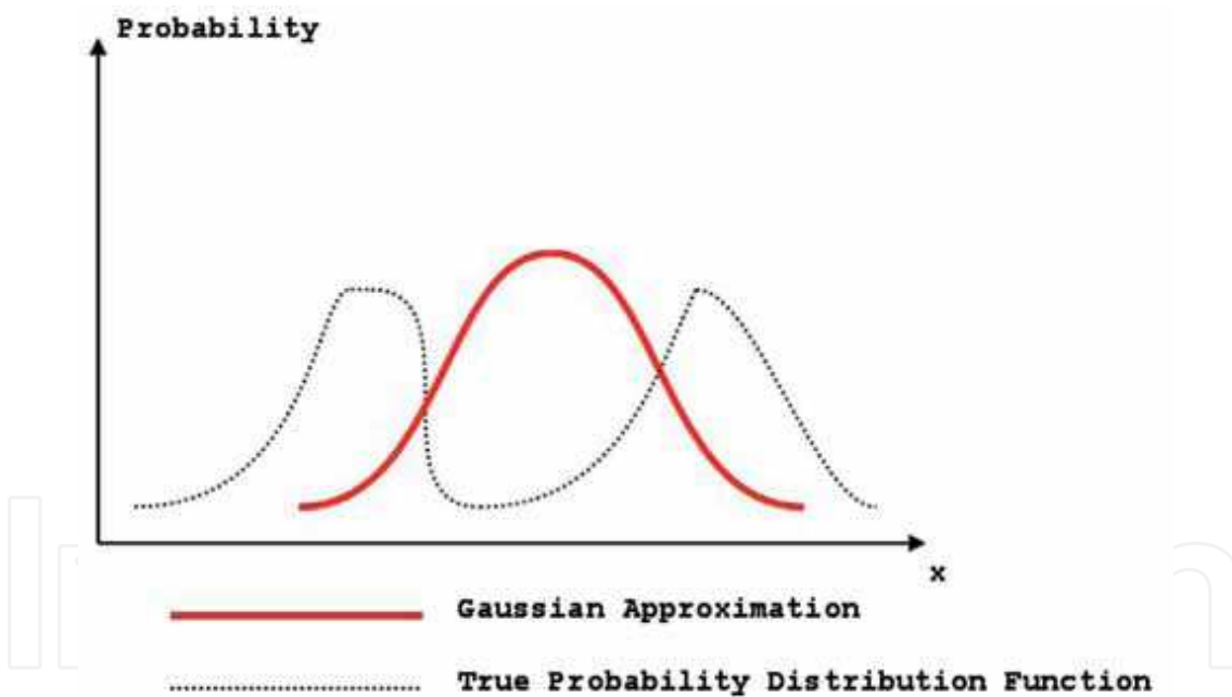
Fig. 3. A single Gaussian approximates a multi-modal probability distribution poorly
