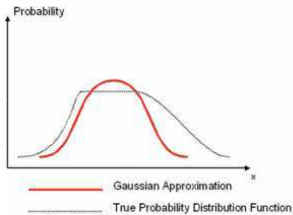
Fig. 1. We approximate a probability distribution function with a uni-modal Gaussian distribution
