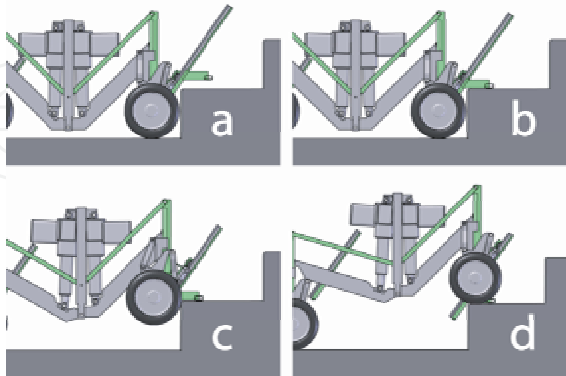
Figure 3. Step climbing process
