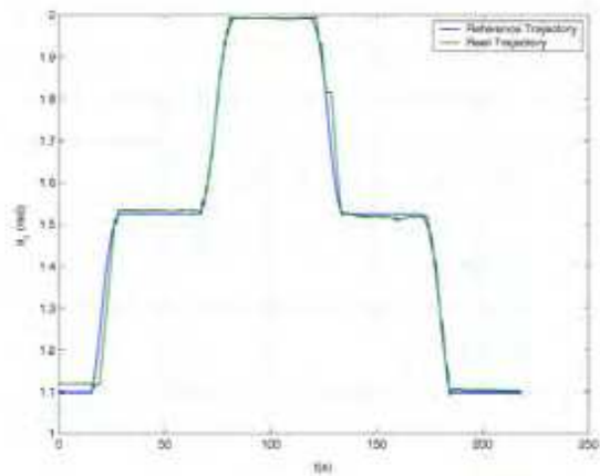
Figure 13. Front joint angle evolution ( \theta_1 ) connected to the chair structure
