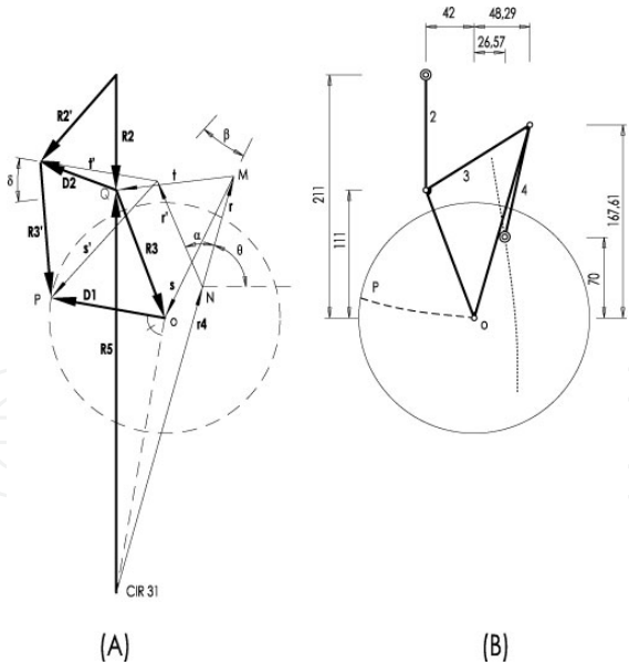
Figure 5. (A) Vector analysis used in the synthesis process of the climbing mechanism. (B) Resulting climbing mechanism
