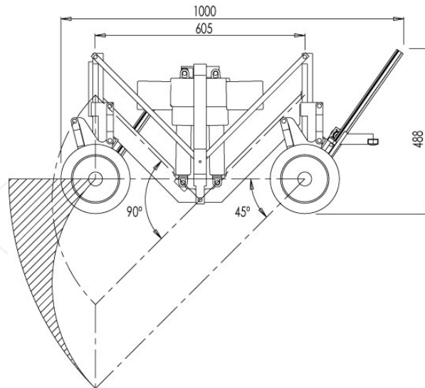
Figure 8. Geometrical parameters and work environment
