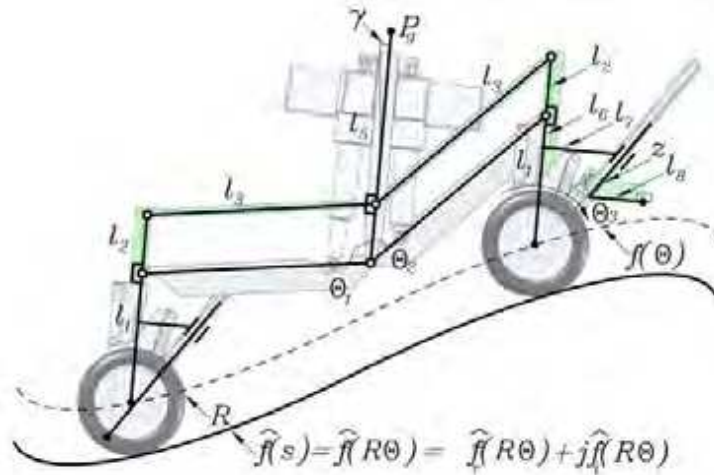
Figure 9. Wheelchair kinematics diagram
