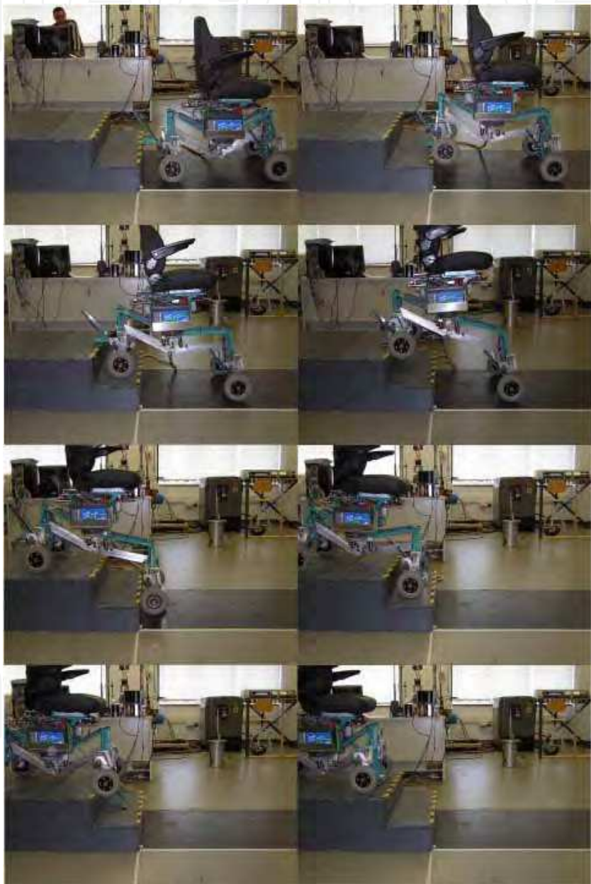
Figure 19. Climbing process sequence
