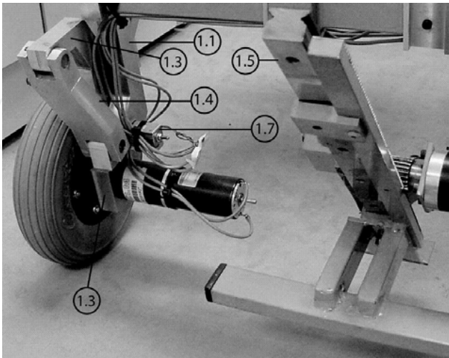
Figure 11. Details of the Climbing Mechanism
