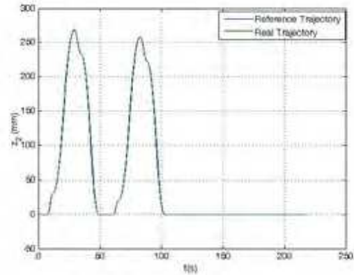
Figure 16. Evolution of the rear climbing mechanism ( z_2 )
