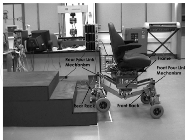
Figure 10. Prototype designed
