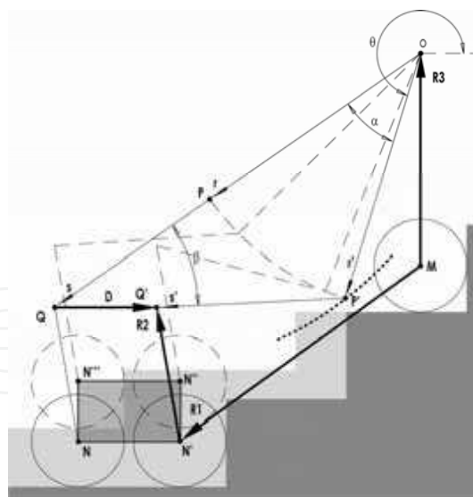
Figure 7. Vector analysis used in the synthesis process of the positioning mechanism
