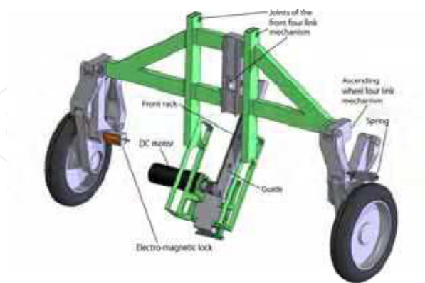
Figure 2. Climbing Mechanism Designed
