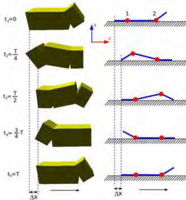
Figure 14. Locomotion of the pitch-pitch (PP) minimal configuration
