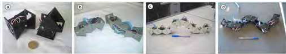
Figure 23. The four robot prototypes built. (a) Y1 modules used to build the robot. (b) The two minimal configurations: PP and PYP. (c) An eight module pitch-connecting modular robot. (d) Pitch-yaw-connecting modular robot with eight modules
