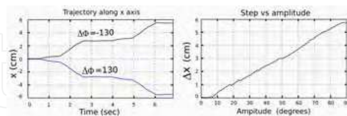
Figure 26. Experiments for the locomotion of the pitch-pitch minimal configuration
