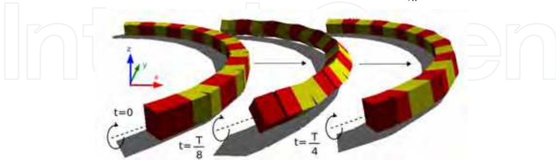
Figure 18. A pitch-yaw connecting robot performing the rolling gait
