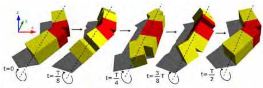
Figure 20. The minimal configuration pitch-yaw-pitch (PYP) performing the rolling gait
