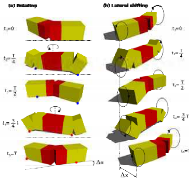
Figure 21. The pitch-yaw-pitch minimal configuration performing the (a) Rotating gait. (b) Lateral shifting
