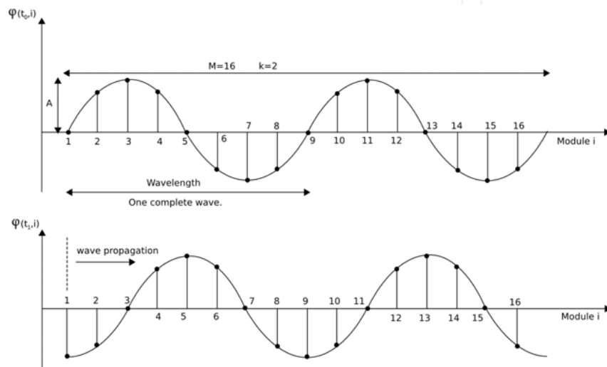
Figure 8. The angular wave at instants t_0 and t_1
