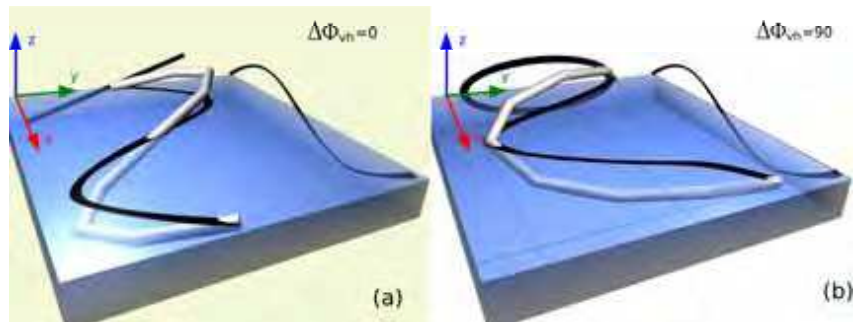
Figure 15. The body wave of the robot as a superposition of its horizontal and vertical body waves
