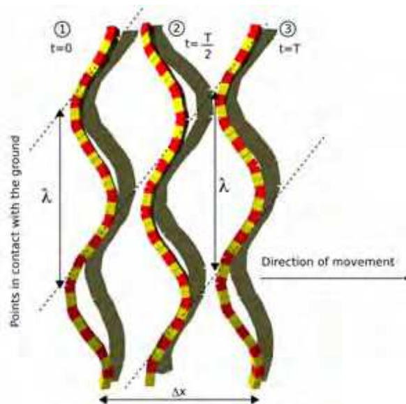
Figure 16. A pitch-yaw connecting robot performing the side winding gait with k_v=k_h=2
