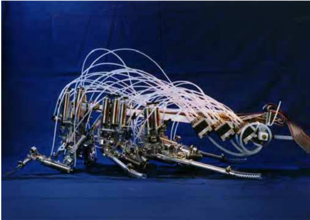
Figure 2. Robot III, a pneumatically powered hexapod modeled structurally and functionally after a cockroach. Robot III was developed at Case Western Reserve University through a long standing collaboration between Roger Quinn's Biorobotics Lab and Roy Ritzmann's neurobiology and behavior lab. Based upon biological data from James Watson, it was designed by Richard Bachmann and Gabriel Nelson with control software by Nelson. (Photo © by and used by permission of R. Quinn. From Quinn et al., 2001, Figure 2, Courtesy of Springer Verlag.)
