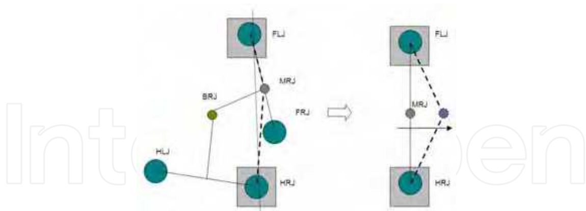
Figure 9. The RGR is represented in its unstable configuration the left; on the right is a schematic representation of the gecko robot, showing the model to be studied for the understanding of its unstable configuration. (FLJ=Fore Left Joint; HRJ=Hind Right Joint; FRJ=Fore Right Joint; HLJ=Hind Left Joint; BRJ=Back Right Joint; MRJ=Middle Revolute Joint.)
