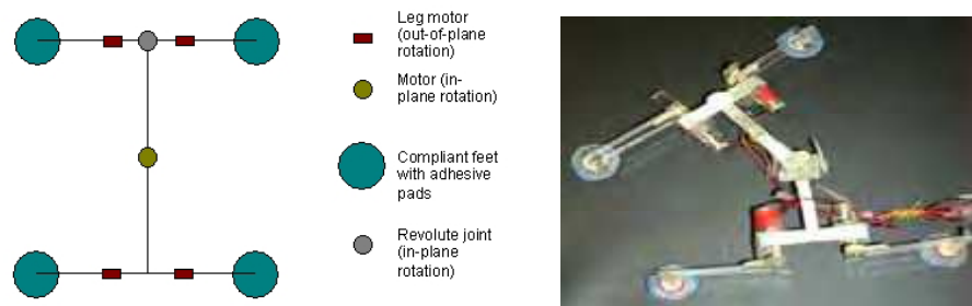
Figure 8. RGR design
