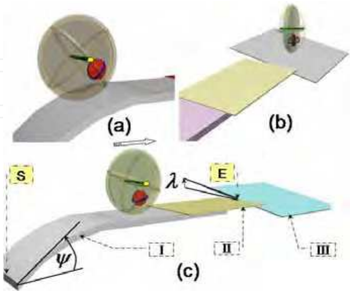
Figure 7. Simulation platform
