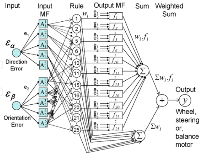
Figure 6. ANFIS architecture
