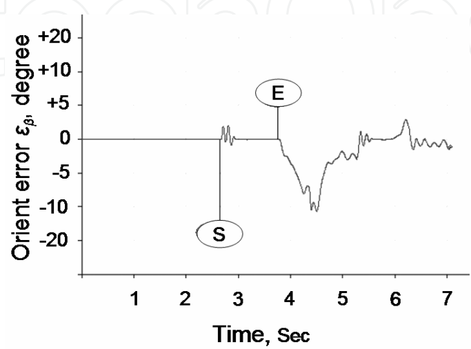
Figure 8 The time variation in orient error angle for \lambda=10^0 and \psi=30^0 under Sugeno control
