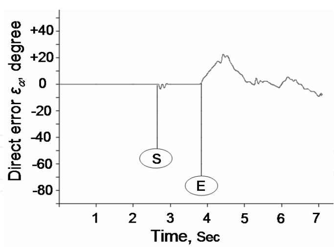
Figure 9 The time variation in direct error angle for \lambda=10^0 and \psi=30^0 under Sugeno control
