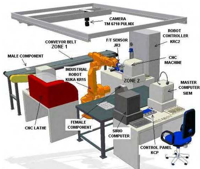
Figure 1. Manufacturing cell
