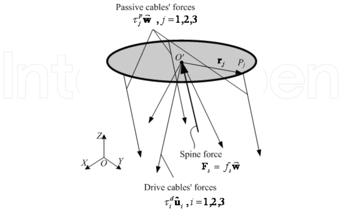
Figure 8. Free body diagram of DishBot 's end-effector
