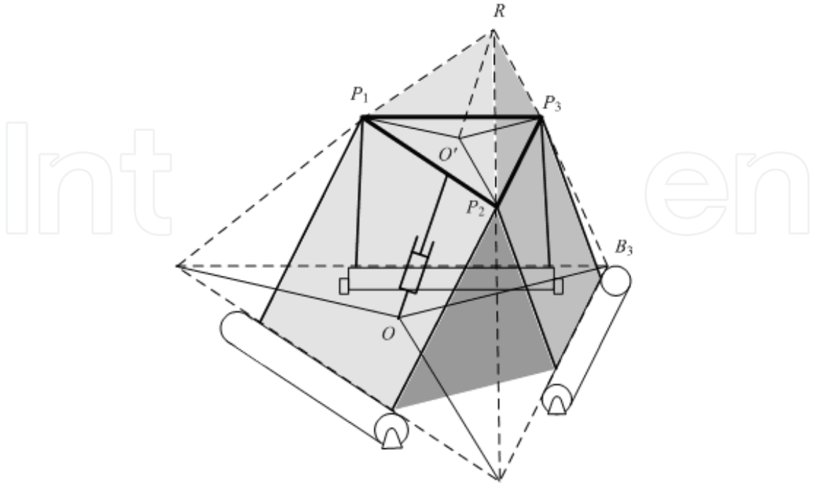
Figure 4. The three planes formed by parallel cables and the spine meet at a point called R .
