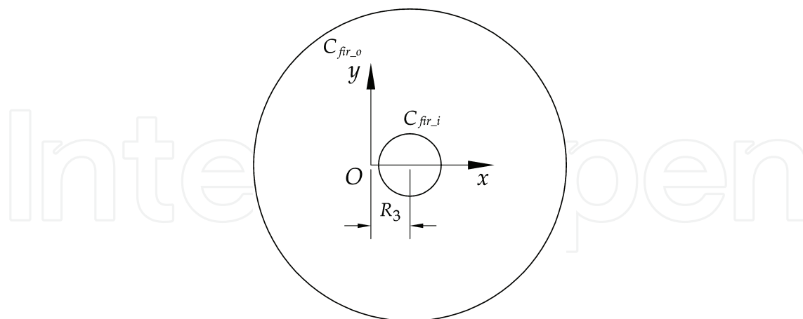
Figure 7. Singular loci of point P when the robot is in the stationary singularity
