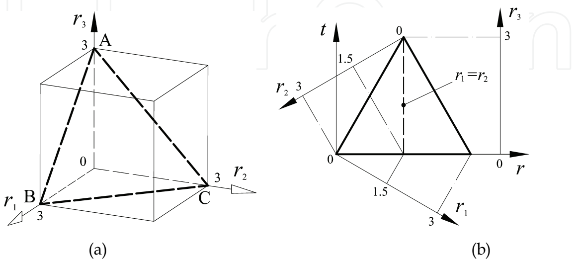
Figure 14. Design space of the 2-DOF translational parallel robot
