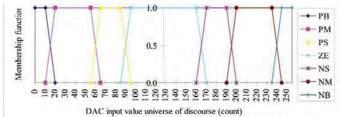
Figure 14. Control action fuzzy set definition.
