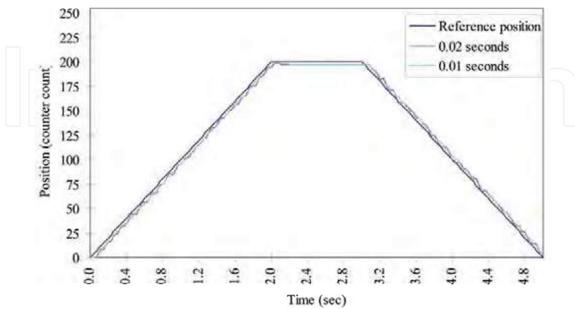
Figure 11. Waist trajectory tracking at different sampling periods.
