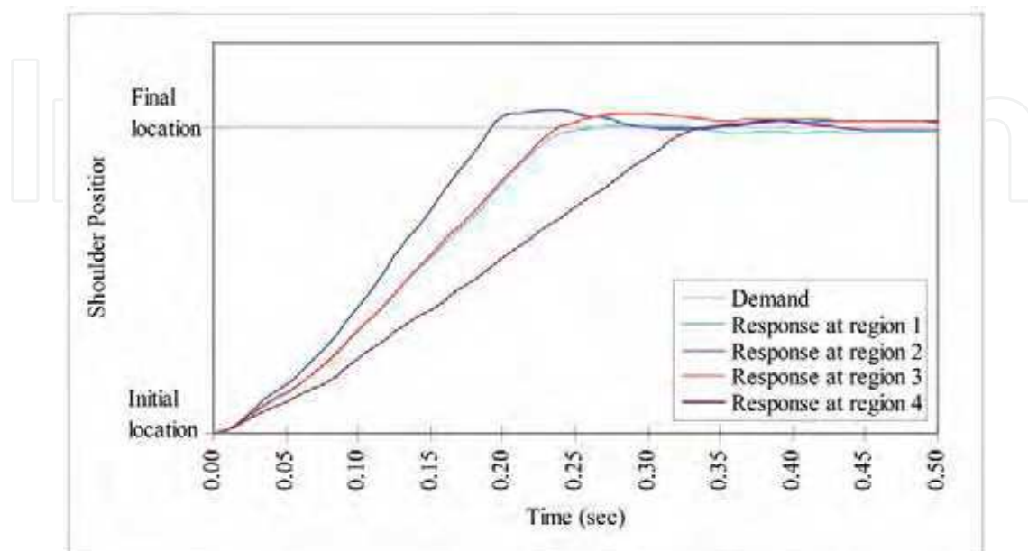
Figure 22. Shoulder response in different regions of operation.
