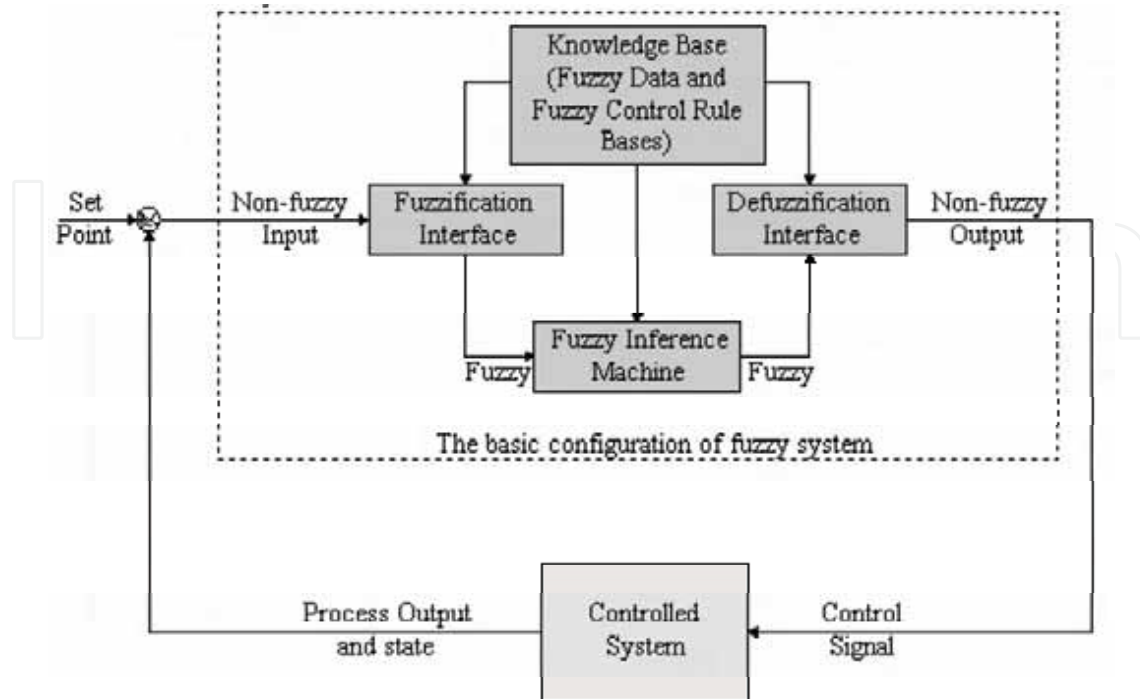
Figure 1. The general form of the fuzzy logic control architecture
