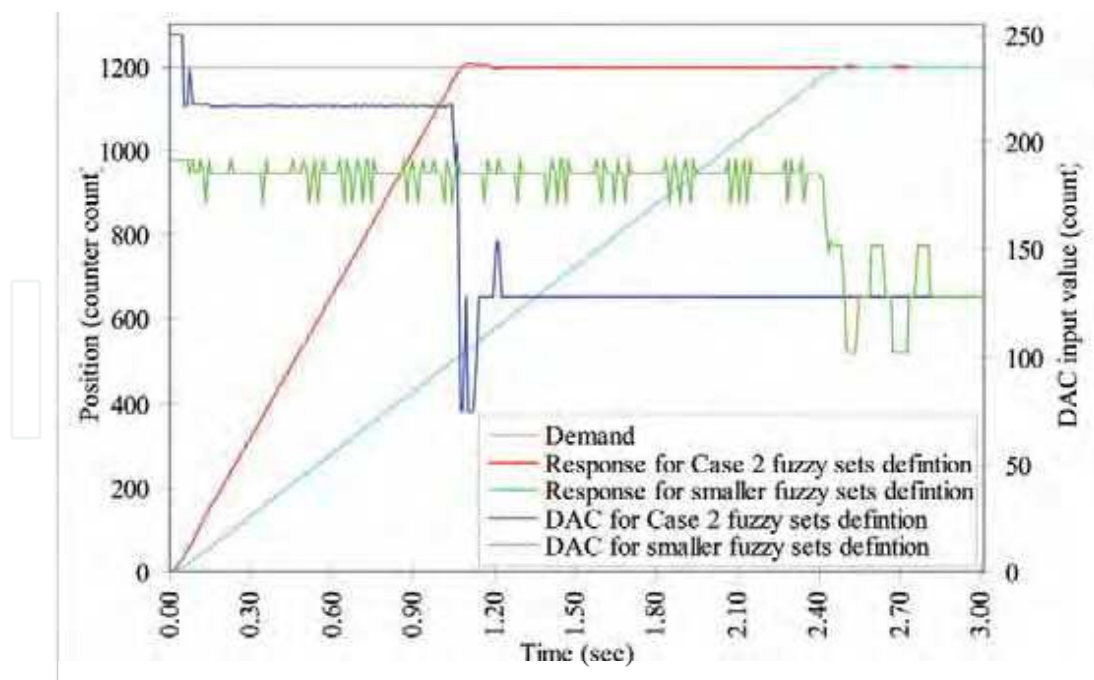
Figure 20. Waist response for different tuned fuzzy sets at second robot arm configuration.
