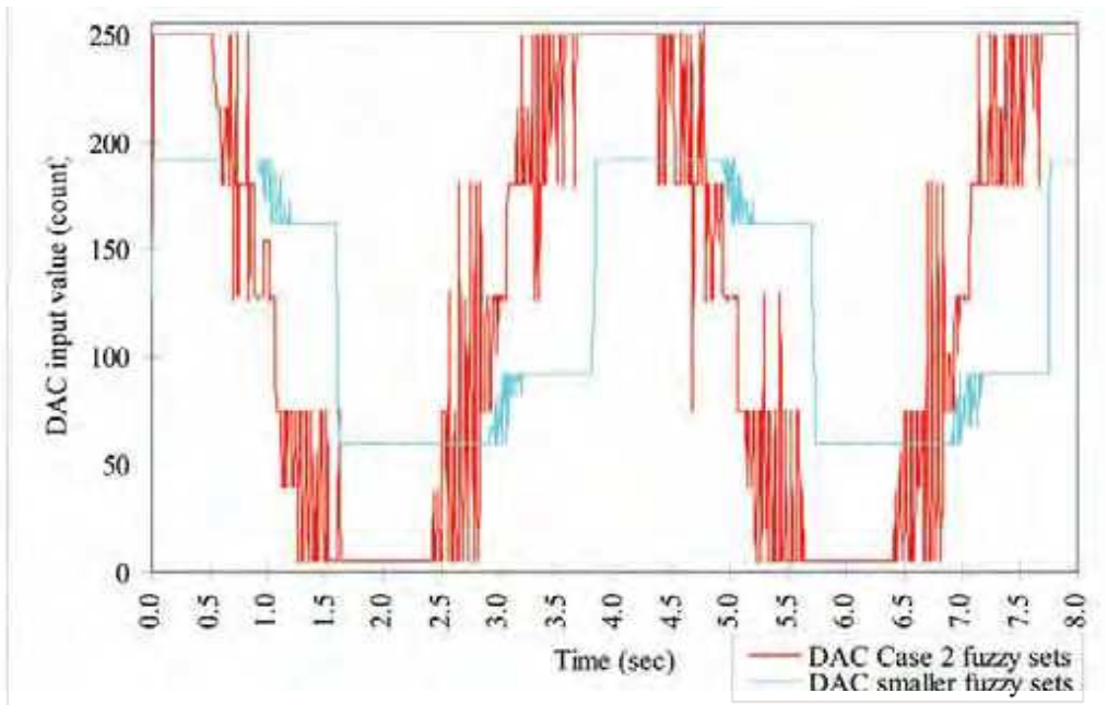
Figure 21(b). Control signal in Fig. 21(a).
