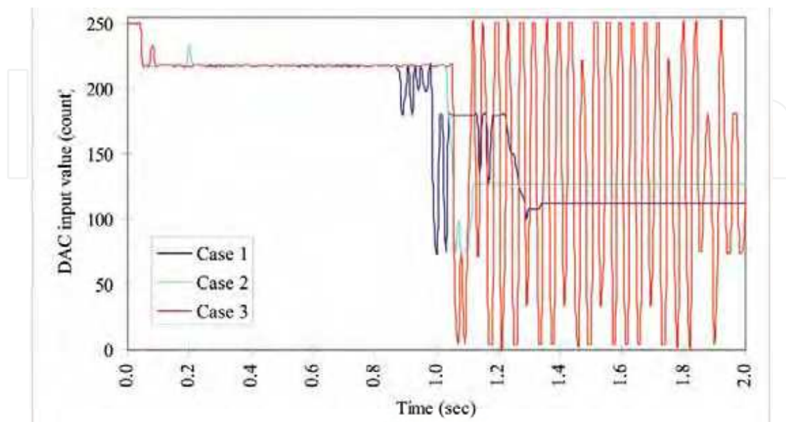
Figure 15(b). Control signals for different error fuzzy set definitions.
