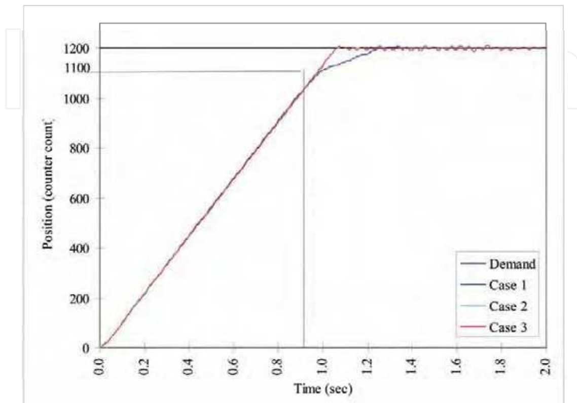
Figure 15(a). Waist response for different error fuzzy set definitions.
