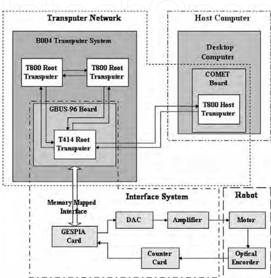
Figure 6. Schematic representation of robot control architecture.
