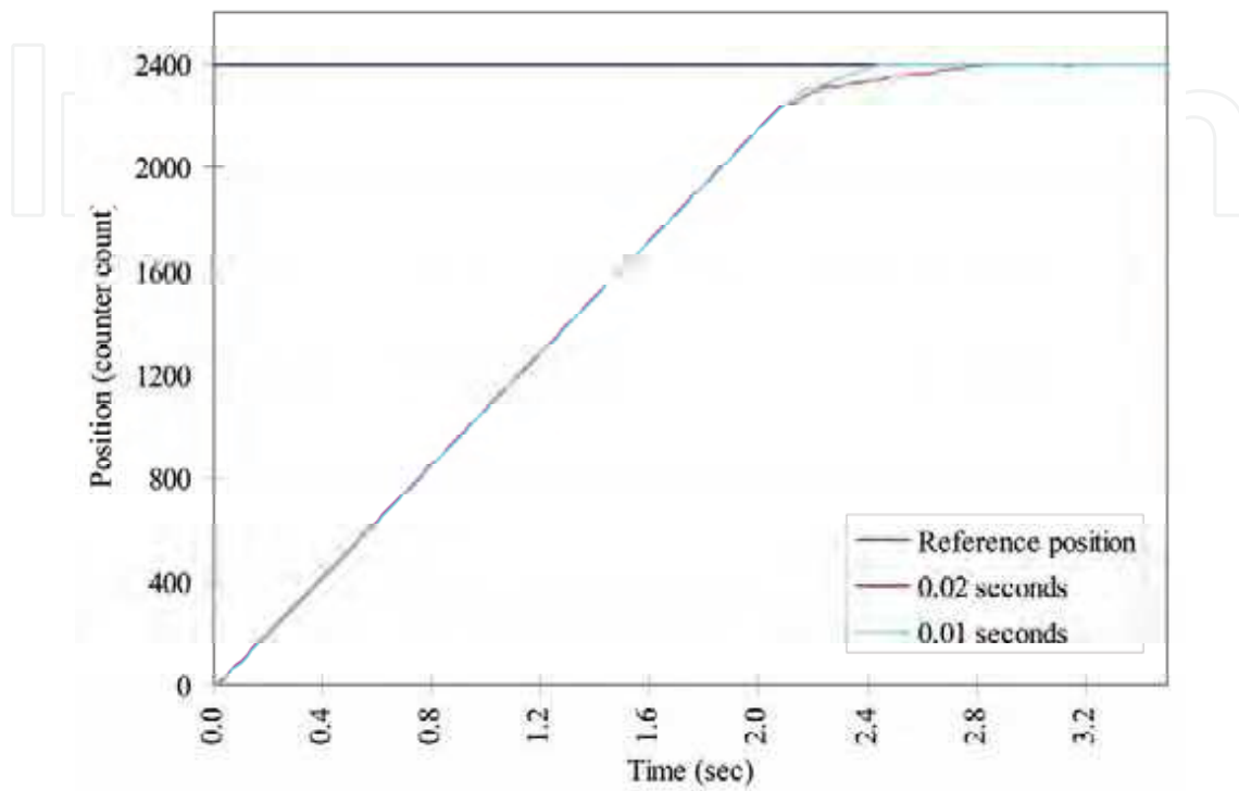
Figure 10. Waist response to a step input for different sampling periods.
