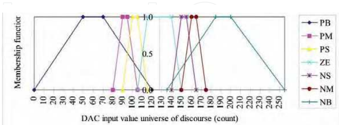
Figure 19. Smaller control action definition of fuzzy sets.
