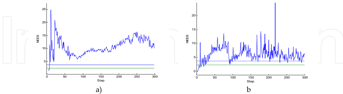
Figure 13. Average NEES of the robot pose (a) (uvd) -observation model (b) UKF
