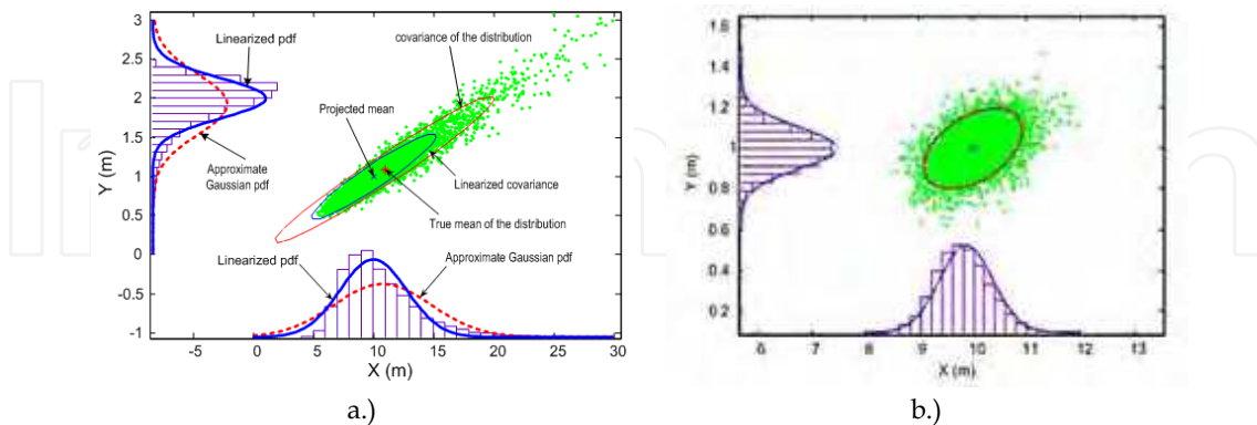
Figure 12. Errors in projective mapping (a) B=0.09\text{m} (b) B=0.5\text{m} , linearized and approximated Gaussians are overlapping
