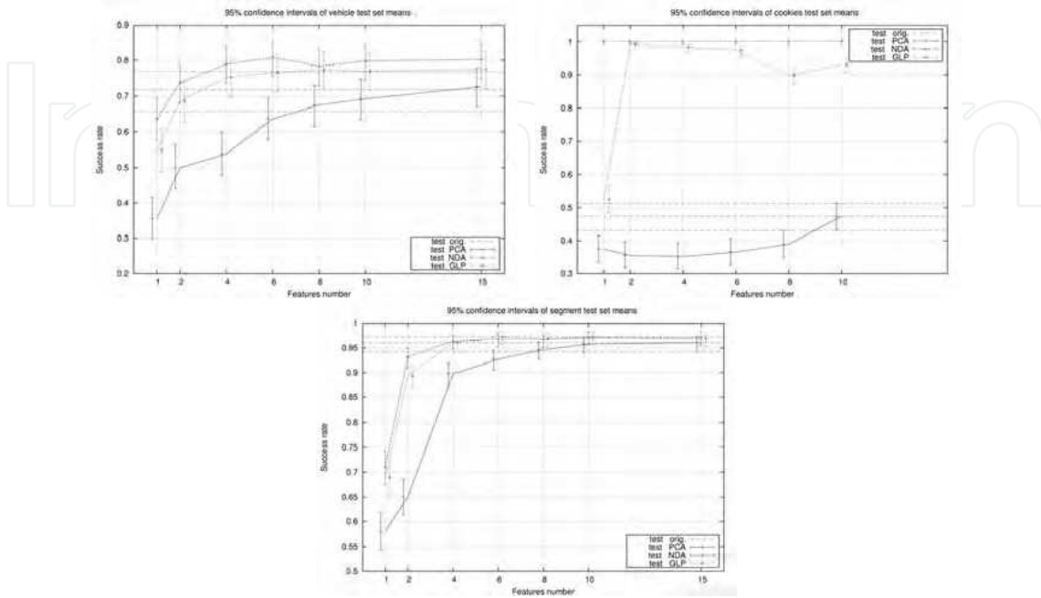
Fig. 1. Correct classification rate results for vehicle (top), cookies (middle) and segment (bottom) data set. The 95% confidence intervals are shown.
