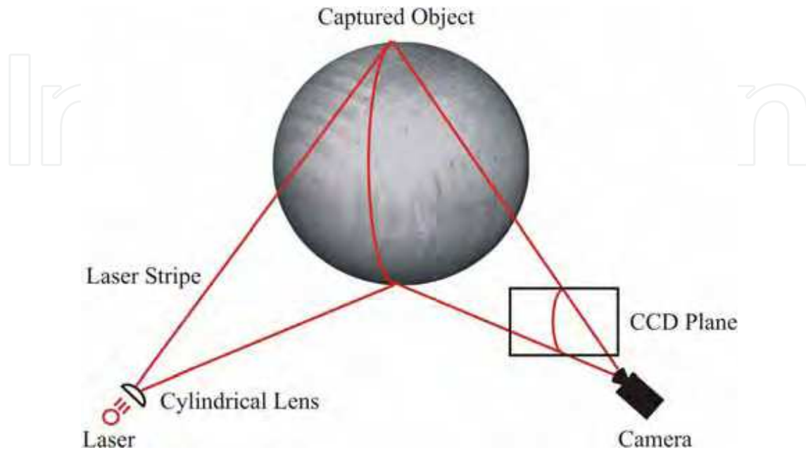
Fig. 2. Optical triangulation using laser beam for illumination.
