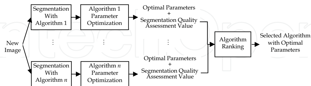
Figure 16. Adaptive static image segmentation schema
