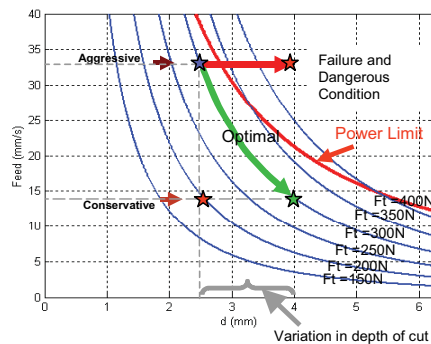
Fig. 20. Controlled material removal rate.
