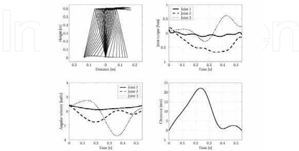
Fig.12. The result of using inequality constraint at intermediate time ( \delta = 20[\text{mm}] , S = 0.150[\text{m}] , T = 0.55[\text{s}] ) (Hase T. & Huang, Q., 2005).
