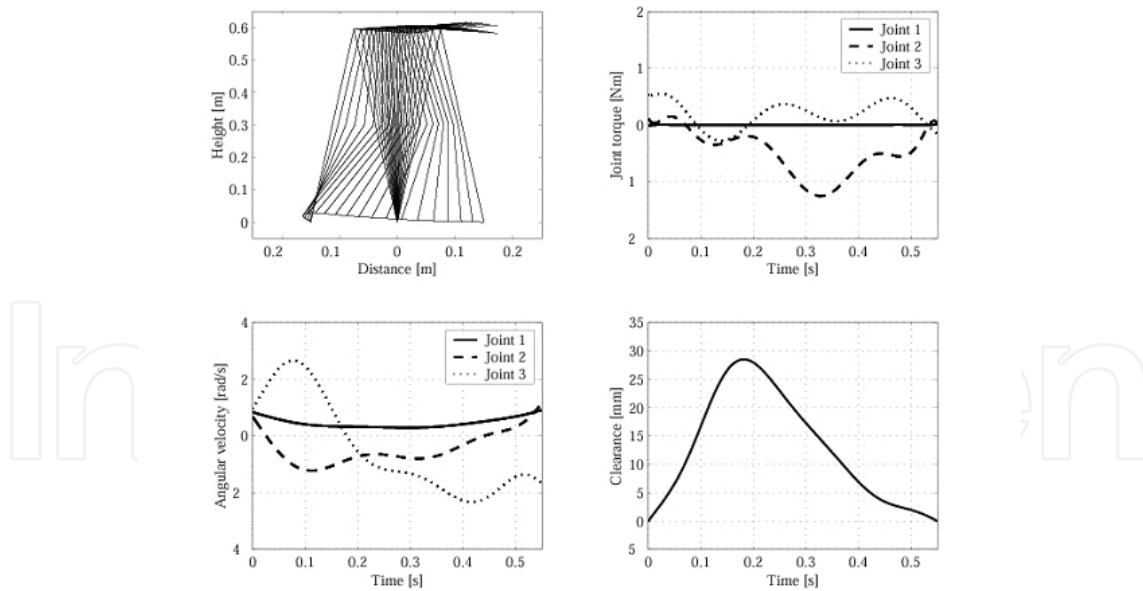
Fig.13. The result of using inequality constraint at intermediate time ( u_1 = 0 , \delta = 20[\text{mm}] , S = 0.150[\text{m}] , T = 0.55[\text{s}] ) (Hase T. & Huang, Q., 2005).
