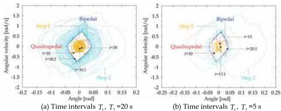
Fig. 8. Roll motion relative to the ground during gait transition from quadrupedal to bipedal locomotion.
