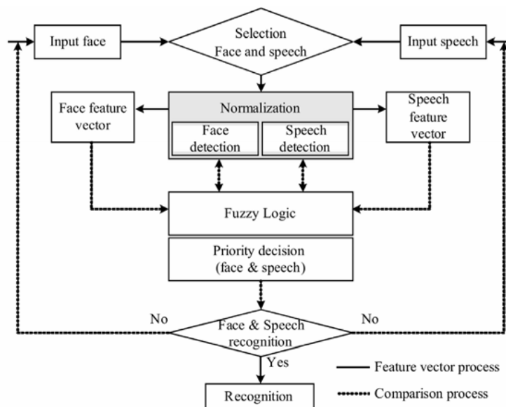
Figure 7. The entire verification process
