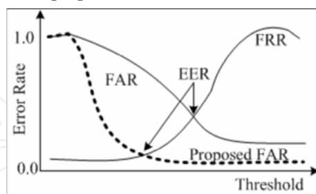
Figure 15. Error rate of the proposed method
