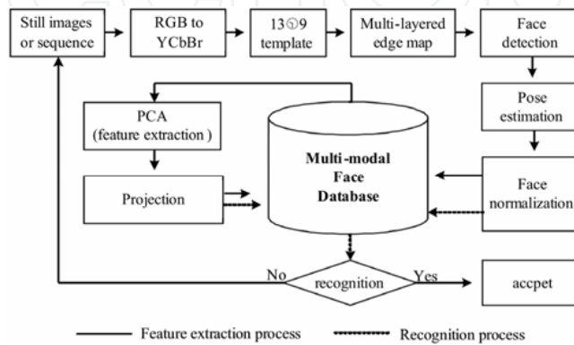
Figure 1. Face feature extraction and recognition process
