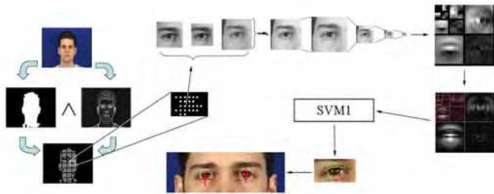
Figure 7. Eye detector outline
