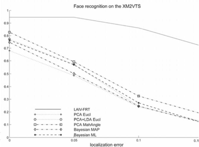
Figure 2. Face recognition vs. (artificial) eye localization precision
