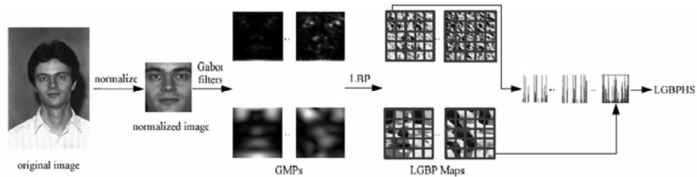
Figure 19. The face pre-processing of CAS-FRT
