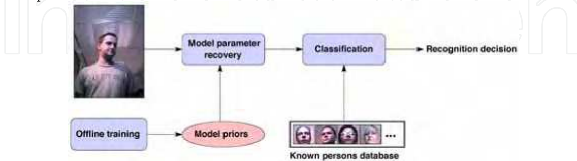
Figure 1. A diagram of the main components of a generic face recognition system. The "Model parameter recovery" and "Classification" stages can be seen as mutually complementary: (i) a complex model that explicitly separates extrinsic and intrinsic appearance variables places most of the workload on the former stage, while the classification of the representation becomes straightforward; in contrast, (ii) simplistic models have to resort to more statistically sophisticated approaches to matching
