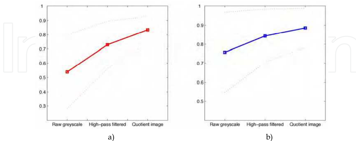
Figure 3. Performance of the (a) Mutual Subspace Method and the (b) Constrained Mutual Subspace Method using raw grey scale imagery, high-pass (HP) filtered imagery and the Self-Quotient Image (QI), evaluated on over 1300 video sequences with extreme illumination, pose and head motion variation (as reported in [3]). Shown are the average performance and \pm one standard deviation intervals
