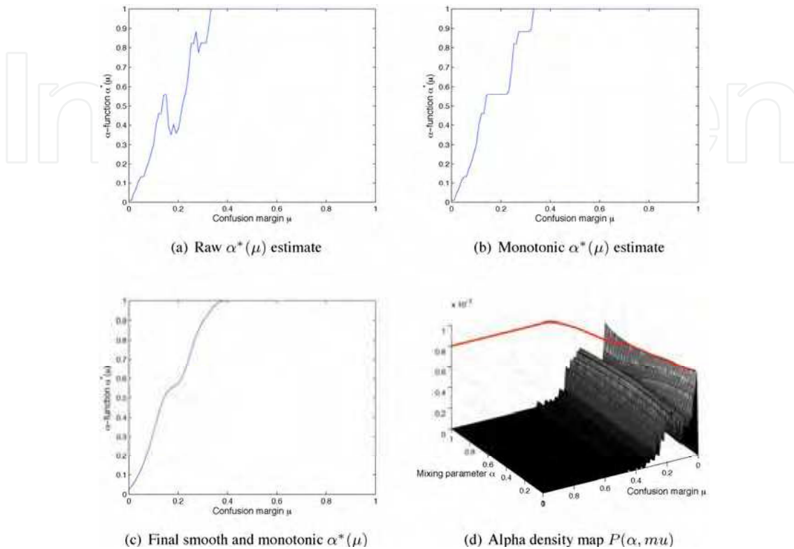
Figure 8. Typical estimates of the \alpha -function plotted against confusion margin \mu . The estimate shown was computed using 40 individuals in 5 illumination conditions for a Gaussian high-pass filter. As expected, \alpha^* assumes low values for small confusion margins and high values for large confusion margins (see (1))
