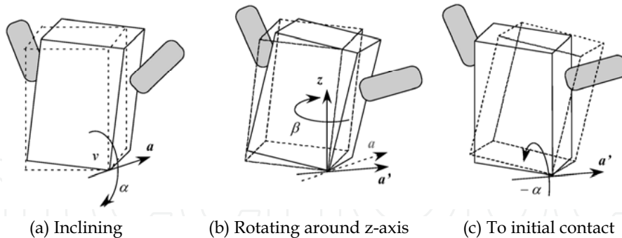
Figure 3. Sequence of pivot motion of a box object composed of three phases, (a) inclination, (b) horizontal rotation and (c) repositioning
