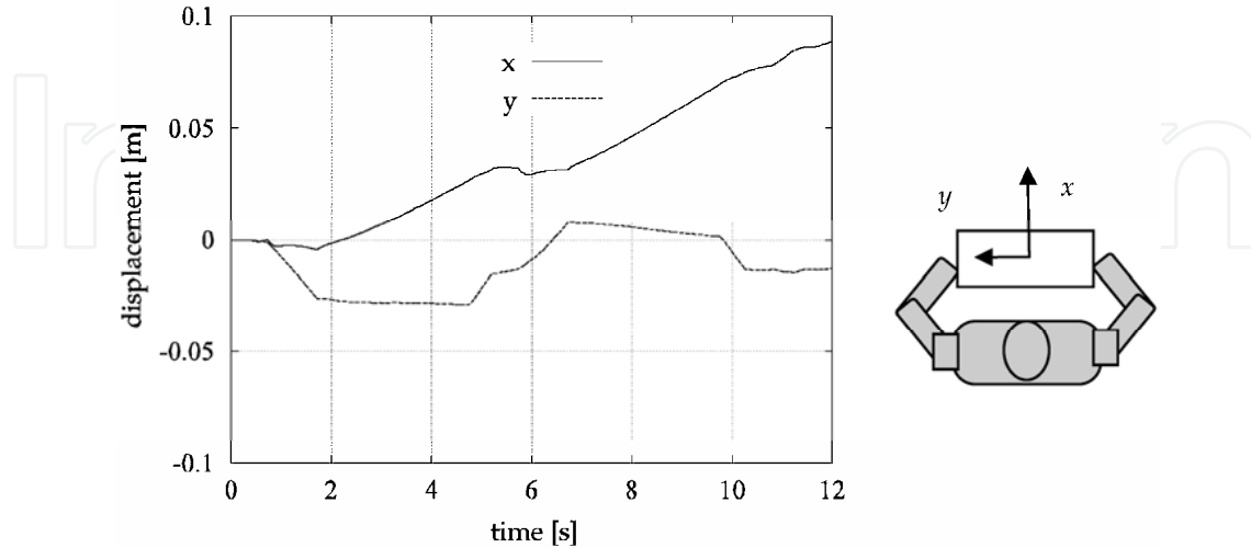
Figure 9. Simulation result of displacement of the center of mass of the manipulated object in x and y directions shown at right-hand side
