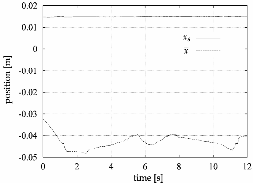
Figure 15. Experimental result of static balancing point ( x_s ) and CoM position ( \bar{x} ). The static balancing point is maintained near the center of the support polygon ( x=0 ) by changing the waist position
