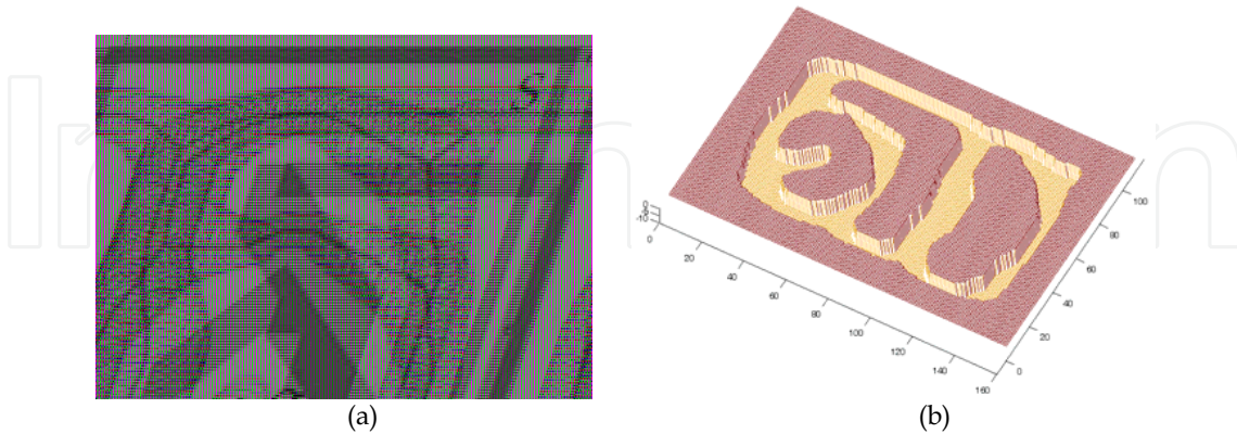
Fig. 16. (a) The PGVG and Region(\alpha MID) (Step P2). (b) Obstacle-free network of valley potentials (Step P3).
