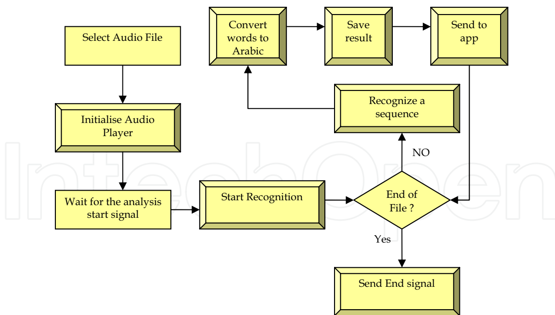
Figure 7. Program Flowchart
