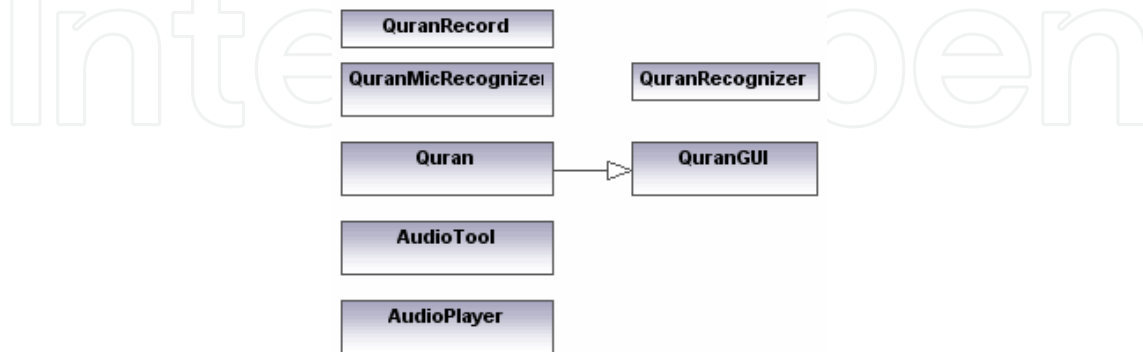
Figure 6. Class Diagram of the Quranic Recognizer application
