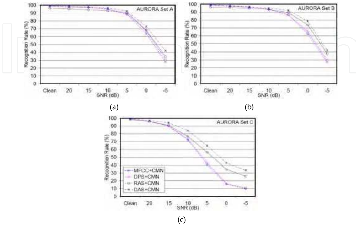
Figure 8. Average recognition accuracies for AURORA 2 multi-condition training. (a) set A, (b) set B and (c) set C. The results correspond to MFCC, DPS, RAS and DAS front-ends with CMN.
