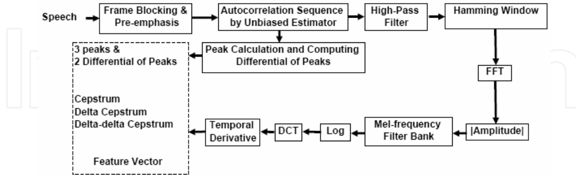
Figure 12. Front-end diagram to extract ACPAF features in autocorrelation domain.
