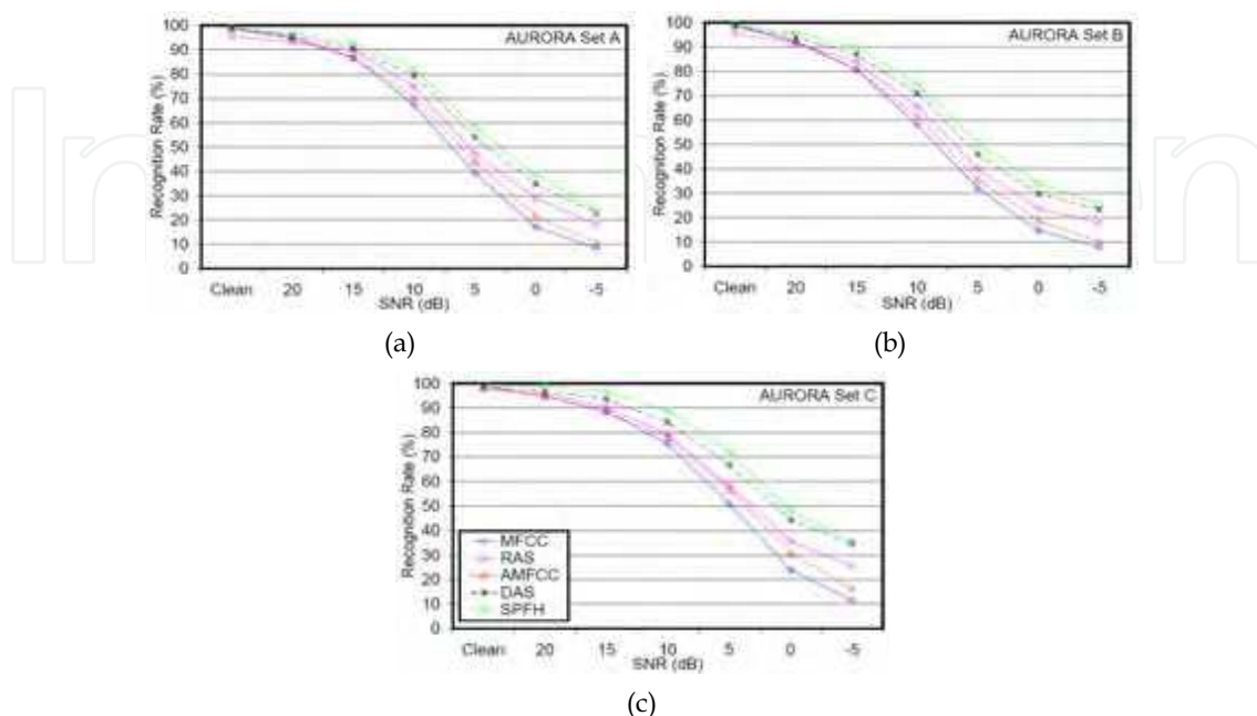
Figure 10. Average recognition rates on Aurora 2 task. (a) Test set a, (b) Test set b, (c) Test set c. The results correspond to MFCC, RAS, AMFCC, DAS and SPFH methods.
