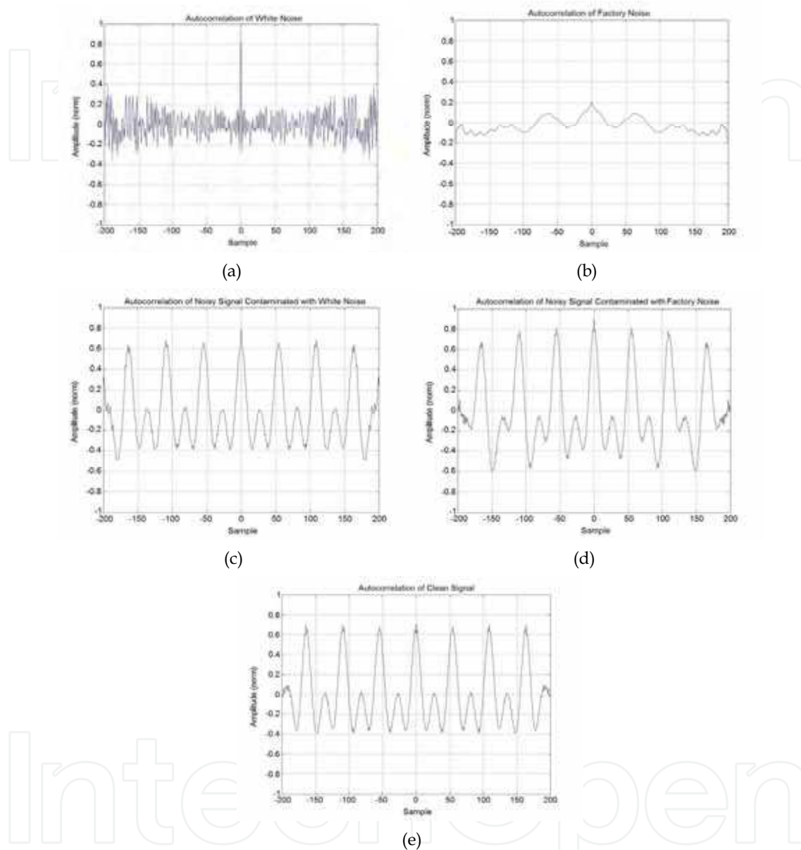
Figure 1. (a) Autocorrelation sequence of white noise, (b) Autocorrelation sequence of factory noise, (c) Autocorrelation sequence for one frame of speech signal contaminated with white noise at 10 dB SNR, (d) Autocorrelation sequence for one frame of speech signal contaminated with factory noise at 10 dB SNR, (e) Autocorrelation of clean speech signal (vowel).
