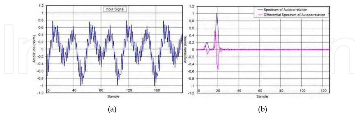
Figure 2. (a) A sample speech signal, and (b) the autocorrelation spectrum magnitude and the differentiated autocorrelation spectrum magnitude of the same signal with a 512-point FFT. Only 128 points of the spectrum are shown for clarity. The sample signal is one frame of phone /iy/ (Farahani et al., 2007).
