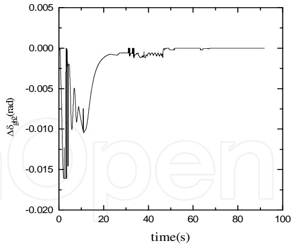
Fig. 29. Output of \Delta\delta_{gb2} .
