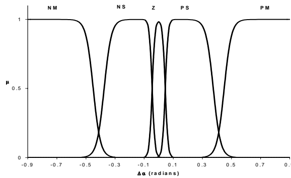
Fig. 9. Membership Functions for Output Variable \Delta\alpha_2 .
