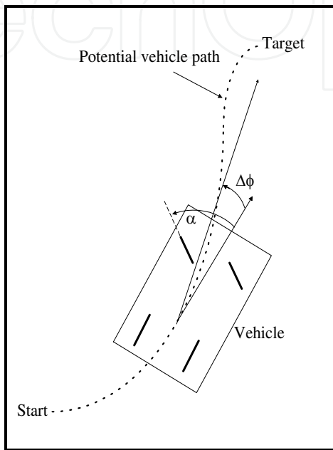
Fig. 4. Input Variables of the Target Steering Module.
