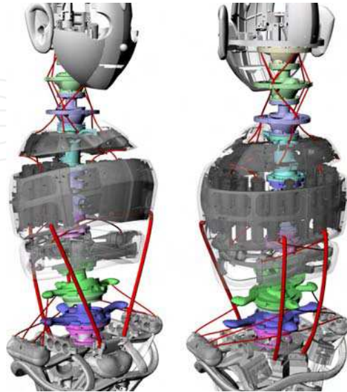
Fig. 4. Bones (gray) and muscles (red) of Kotaro's torso.
