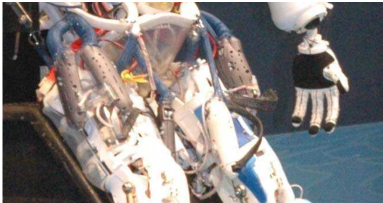
Fig. 3. The muscle units attached around both crotch joints.
