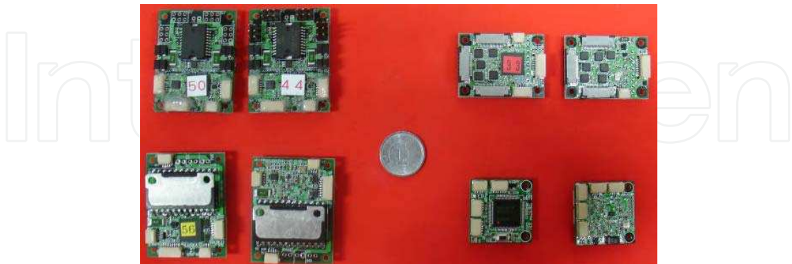
Fig. 14. Developed circuit boards (upper-left: for 4 small motors, lower-left: for 2 middle motors, upper-right: for 384 analog sensors, lower-right: 7-port USB2 hubs).
