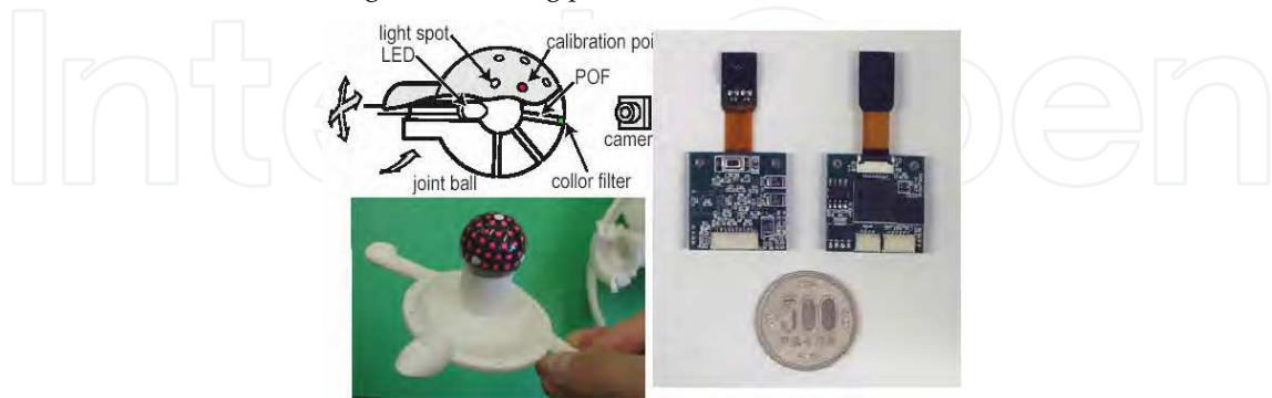
Fig. 13. Posture sensor for ball-and-socket joint using a mobile phone camera and a mobile phone microprocessor.
