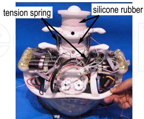
Fig. 6. Elastic and viscous elements between joints.
