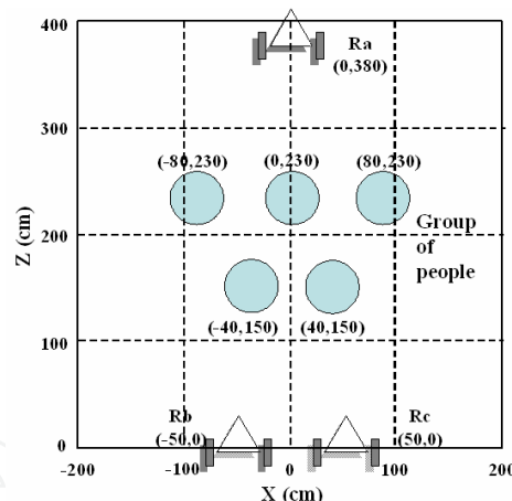
Figure 5. Experiment configuration with 5 people, and 3 mobile robots
