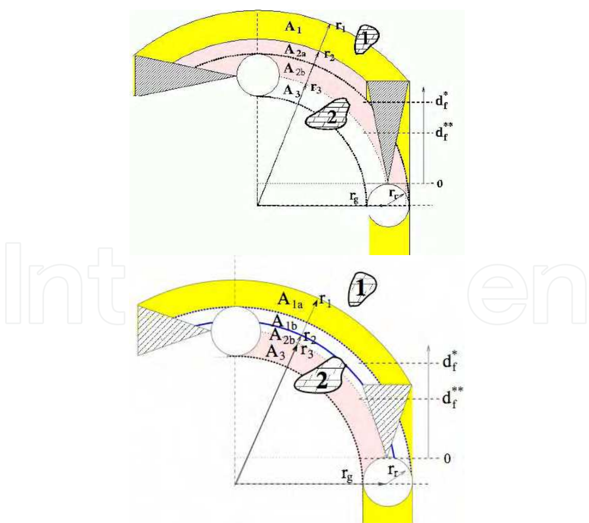
Figure 3. Robot turning with constant velocities. Its sensor Field of Regard fulfills conditions (4) and (6). (Left) Case when d_f > d_f^* and the tunnel vision problem: the robot moves where the sensors did not reach. (Right) For d_f^{**} > d_f > d_f^* the situation is better, but still there are blind zones
