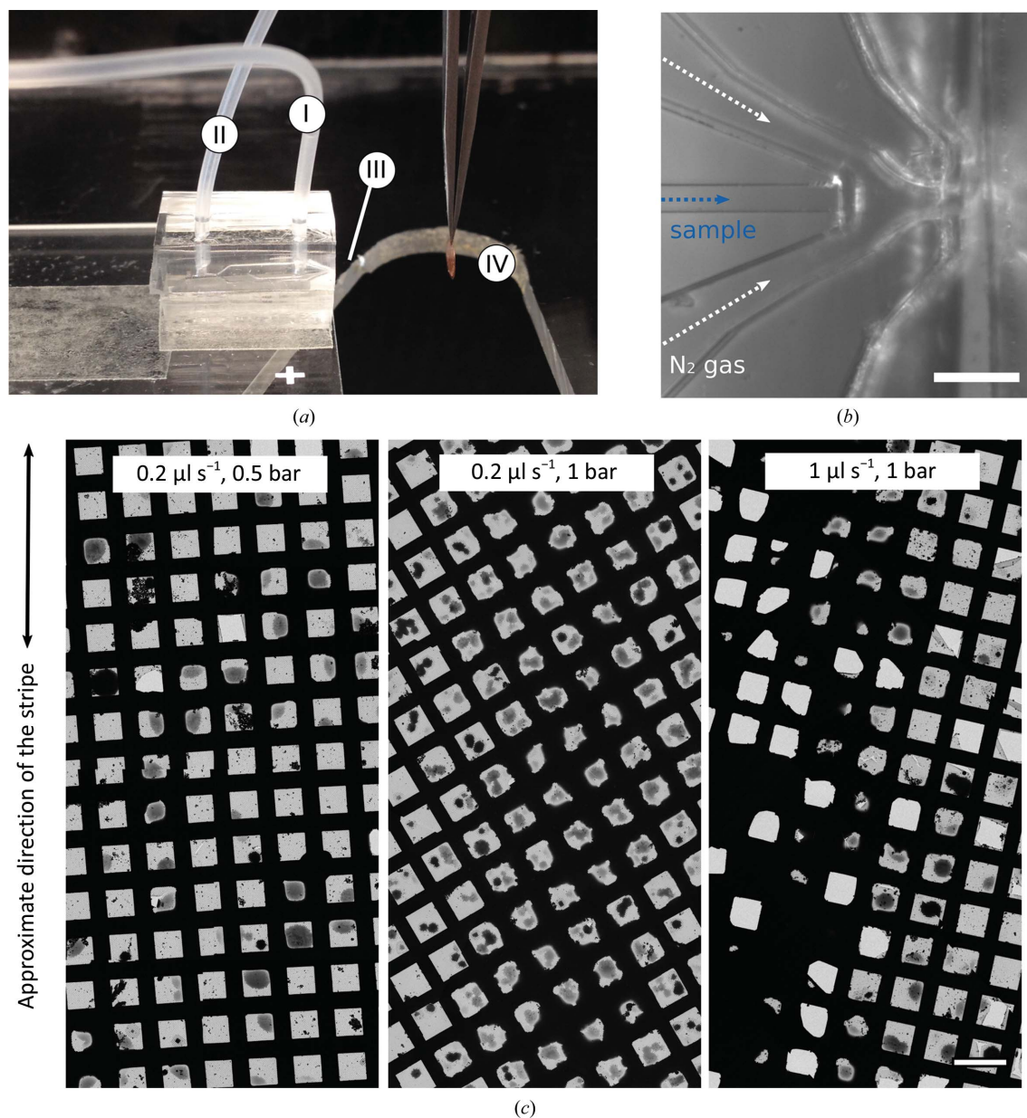
Figure 3 GDVN used for cryo-EM grid preparation. (a) The GDVN device fitted within the current setup showing (I) the liquid inlet tubing, (II) the \text{N}_2 gas inlet tubing, (III) the position of the nozzle and (IV) the grid in the target position for spraying. (b) Microscopic image of the internal GDVN geometry used in this work with the sample and gas channels labelled. The scale bar denotes 100 \mu\text{m} . (c) Typical grids generated with the microfluidic GDVN device under three different conditions. On all three grids, liquid was deposited approximately as a stripe across the grid. The scale bar denotes 100 \mu\text{m} .
