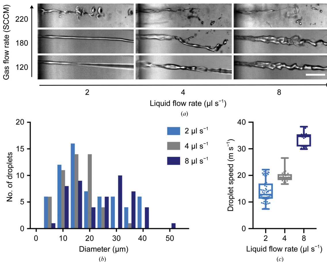
Figure 4 (a) High-speed imaging at the GDVN orifice of the jet/spray transition resulting from increasing gas and liquid flow rates. Bursts of 3000 consecutive frames were collected at 200 000 frames per second (fps) with an exposure time of 10 ns (pulsed laser illumination). The scale bar is 100 \mu\text{m} . (b) Droplet diameter distribution for a 220 SCCM \text{N}_2 flow. (c) Droplet-speed distribution at 220 SCCM.
