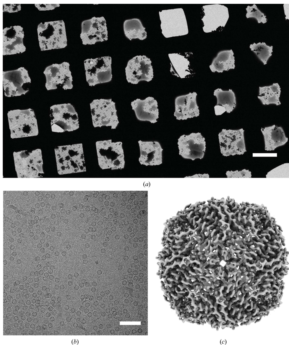
Figure 5 (a) Low-magnification cryo-electron micrograph of a grid prepared using the microfluidic GDVN device in spraying mode (liquid at 4 \mu\text{l s}^{-1} , gas at 2 bar). The scale bar corresponds to 50 \mu\text{m} . (b) Representative high-magnification image of an area with thin ice used for data collection (the scale bar corresponds to 50 \text{nm} ). (c) Single-particle reconstruction of apoferritin to 3.5 \text{Å} resolution with data collected from a single grid made using the GDVN nozzle under spraying conditions (liquid at 4 \mu\text{l s}^{-1} , gas at 2 bar).
