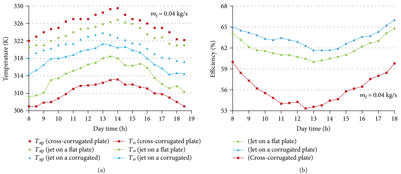
FIGURE 18: Hourly performance parameters under the purview of three designs of solar air heater. (a) Absorber plate temperature and air outlet temperature. (b) Collector efficiency.
