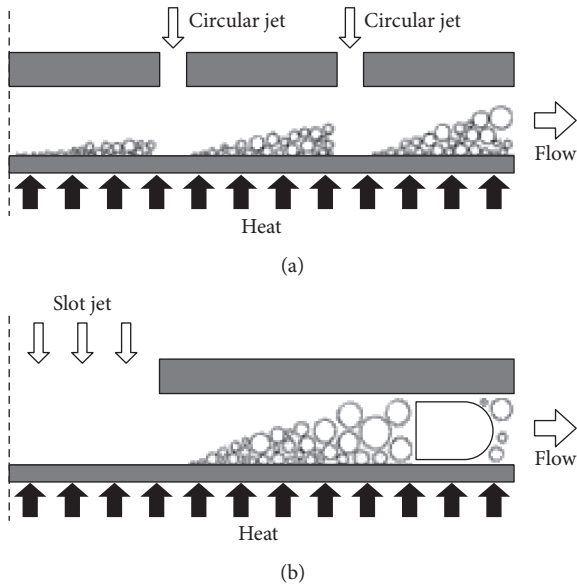
FIGURE 5: Two different jets. Multiple circular jets and single-slot jet [33].
