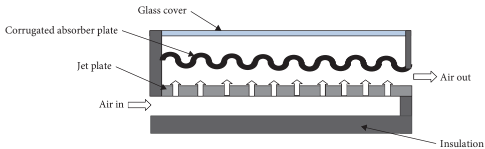
FIGURE 11: Schematic diagram of the proposed design of SAH with jet impingement on a corrugated absorber plate.
