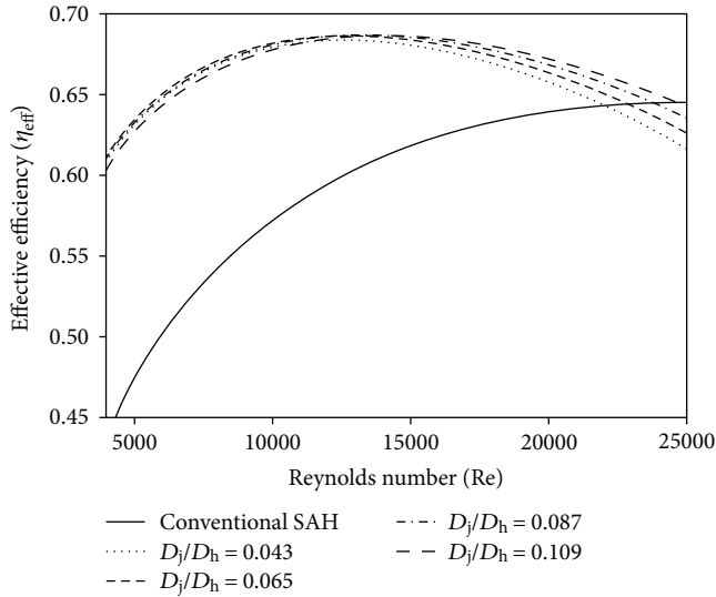
FIGURE 8: Variation of effective efficiency with Reynolds number at different values of jet diameter ratio [7].
