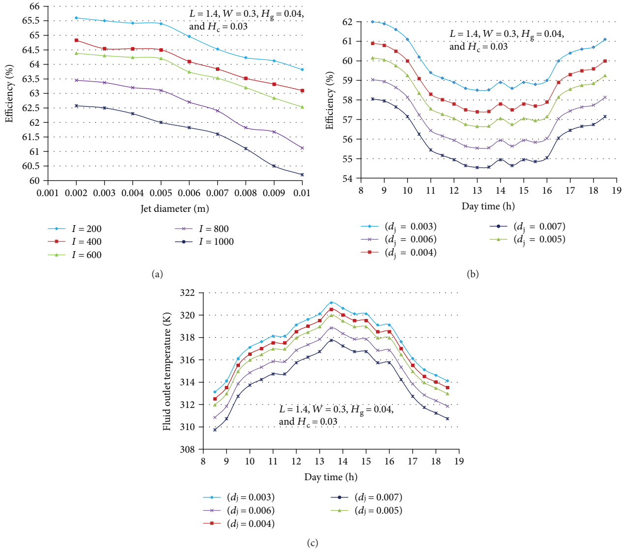
FIGURE 21: Prediction of the optimum jet diameter ( d_j ) of the proposed solar air heater. (a) SAH efficiency versus jet diameter at different solar radiation levels. (b) Hourly SAH efficiency over daytime at different jet diameters. (c) Hourly air outlet temperature at different jet diameters.
