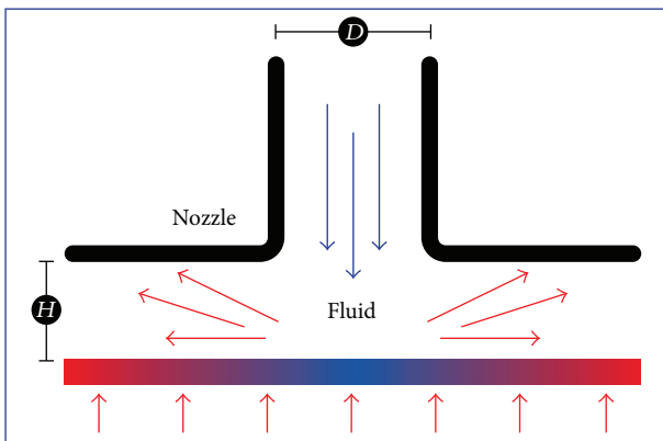
FIGURE 4: Effect of directed fluid released against the heat transferring surface.
