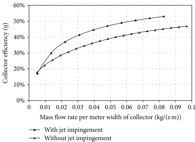
FIGURE 6: Efficiency at typical conditions of the collector with and without jet impingement [34].
