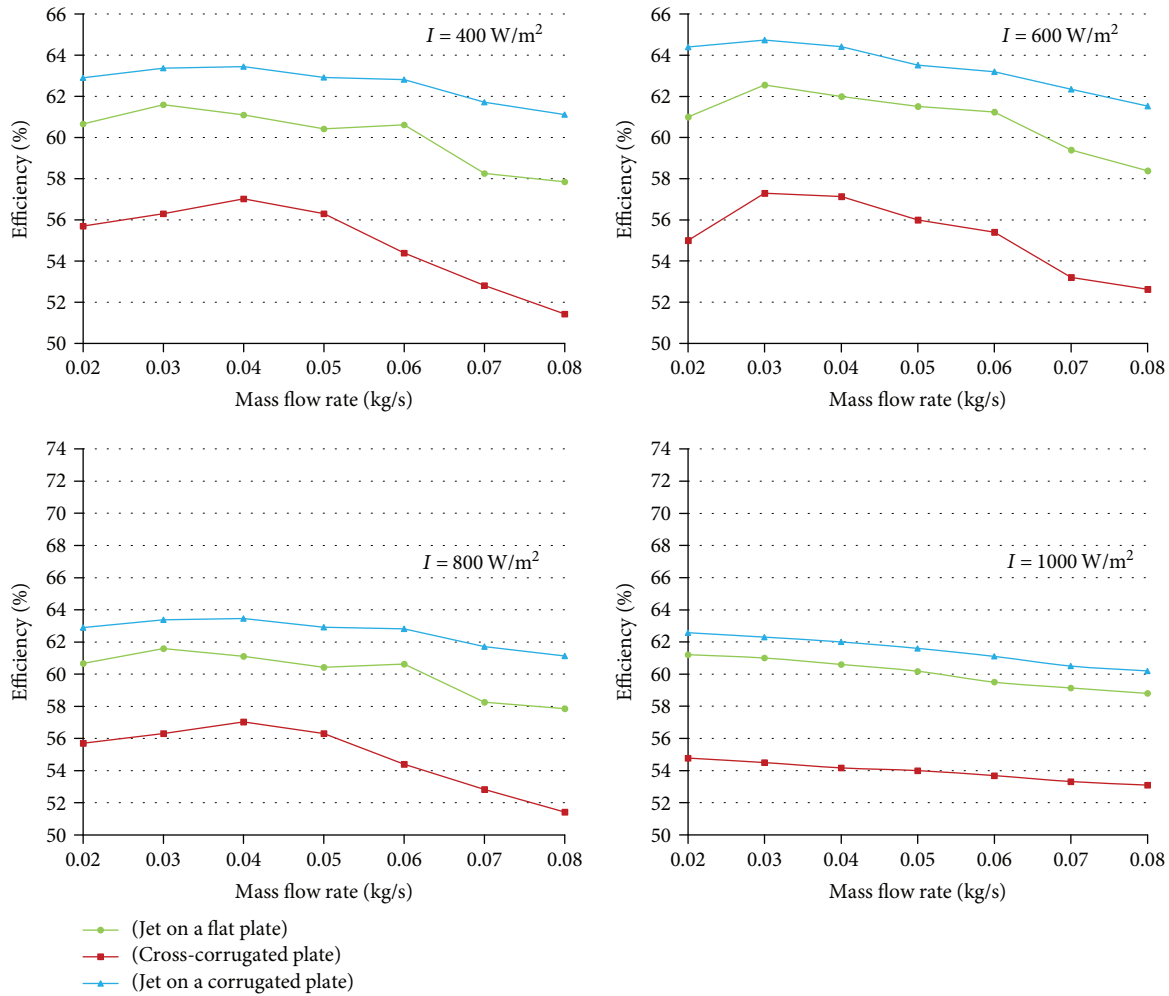
FIGURE 17: SAH Efficiency under the purview of three collector designs versus mass flow rate for different solar radiation levels.
