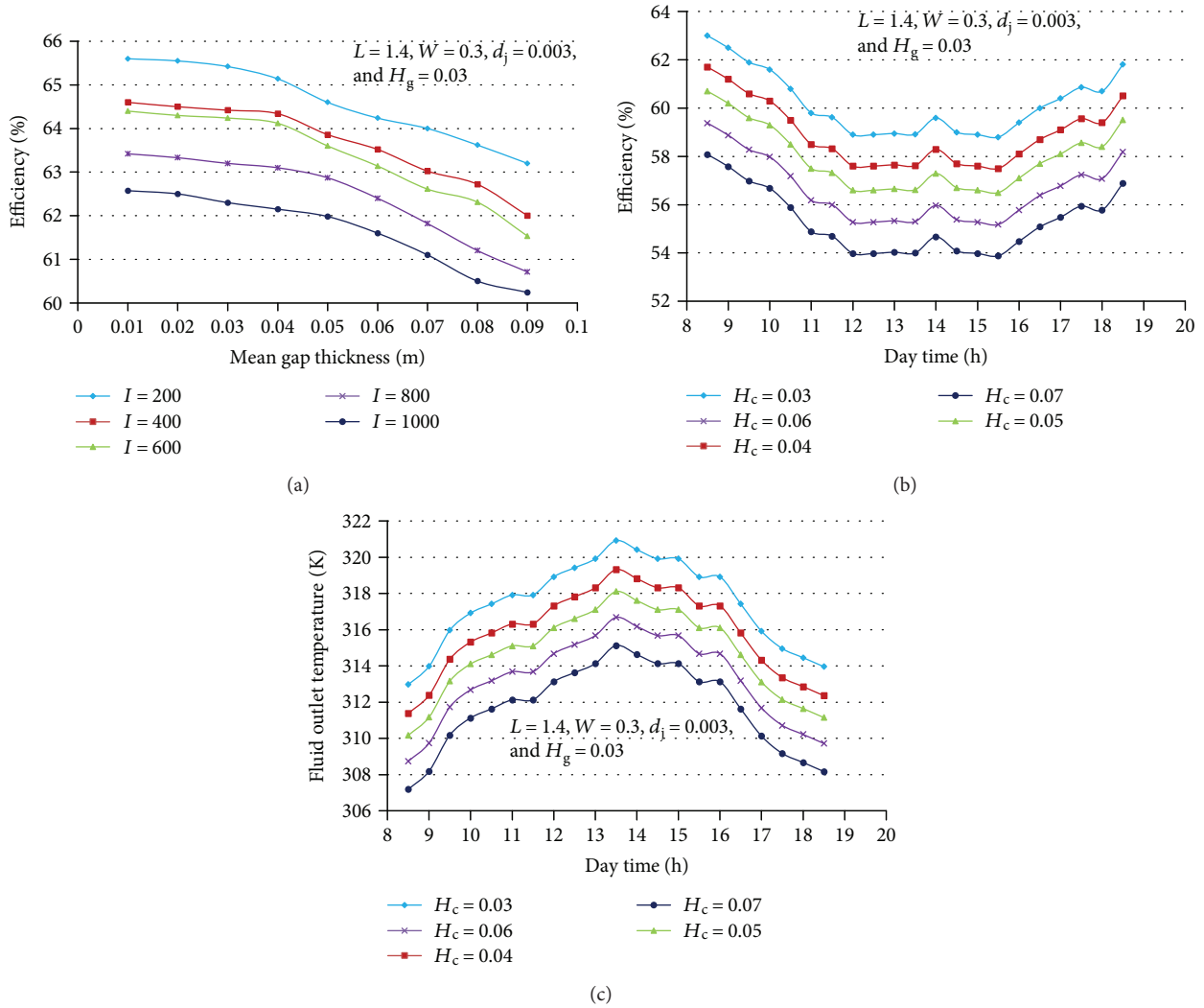
FIGURE 23: Prediction of the optimum mean gap thickness between the absorber plate and the glass cover ( H_c ) of the proposed solar air heater. (a) SAH efficiency versus H_c at different solar radiation levels. (b) Hourly SAH efficiency over daytime at different H_c . (c) Hourly air outlet temperature at different H_c .
