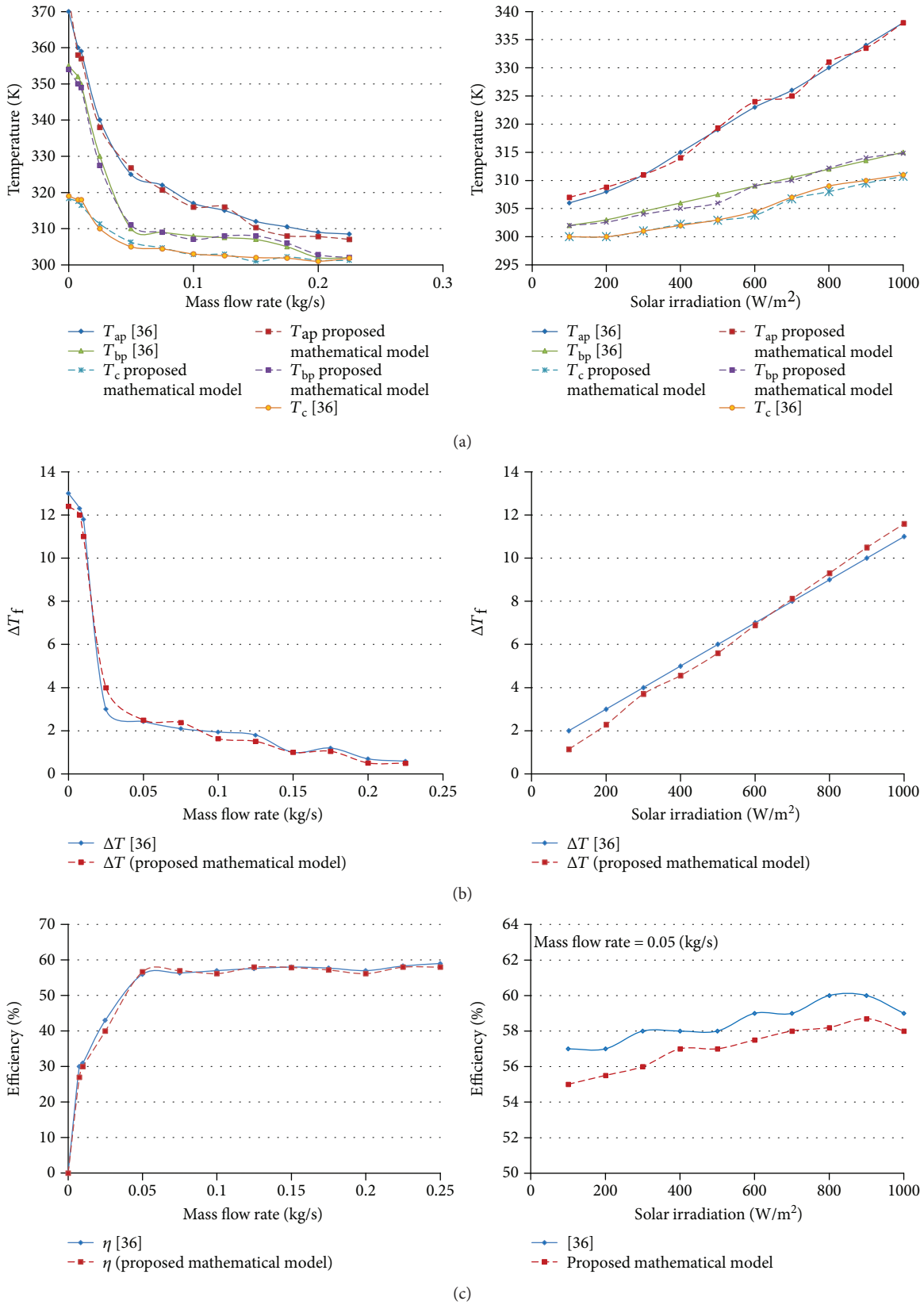
FIGURE 14: Comparison of solar air heater performance parameters obtained from the proposed mathematical model and that in [36]. (a) Predicted temperature of absorber plate, bottom plate, and glass cover plate of SAH versus mass flow rate and solar irradiation. (b) Predicted fluid temperature difference versus mass flow rate and solar irradiation. (c) Predicted SAH efficiency versus mass flow rate and solar irradiation.
