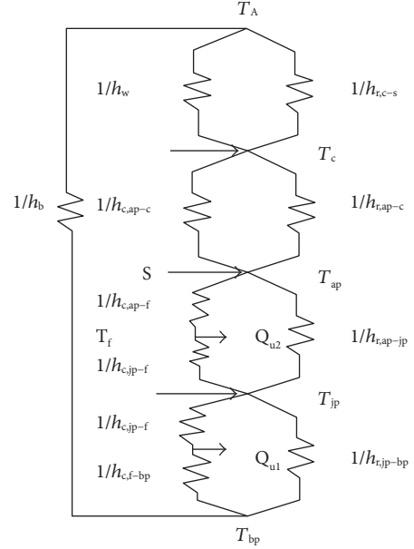
FIGURE 13: Thermal network for the single-cover solar air heater.
