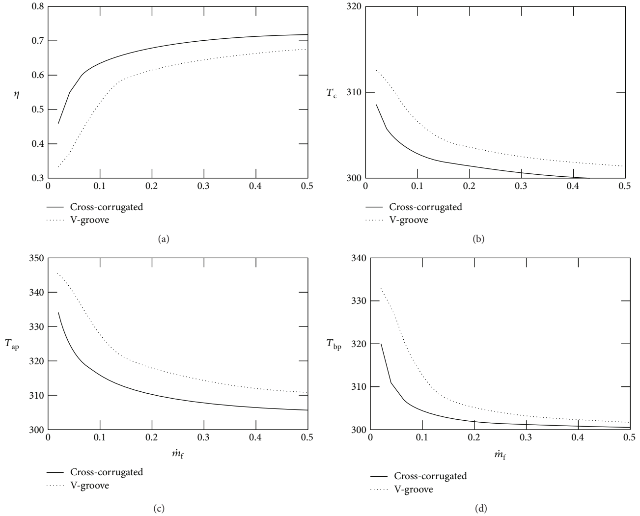
FIGURE 3: (a–d) Efficient heat removal by cross-corrugated compare to V-groove collector, Liu et al. [28].
