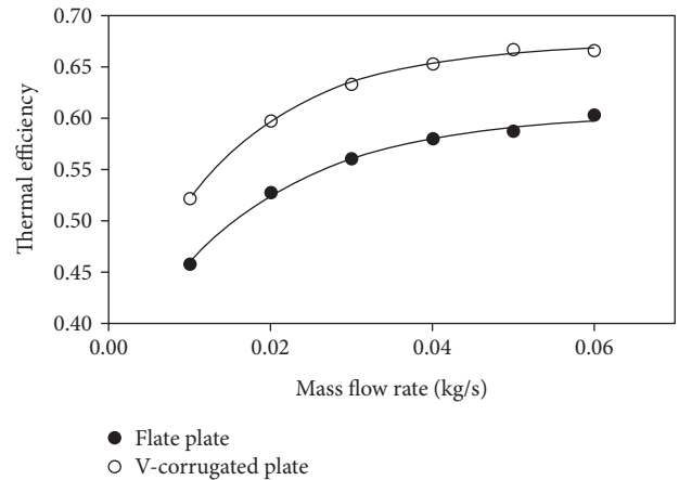
FIGURE 1: Effect of mass flow rate of flat and corrugated plates [26].
