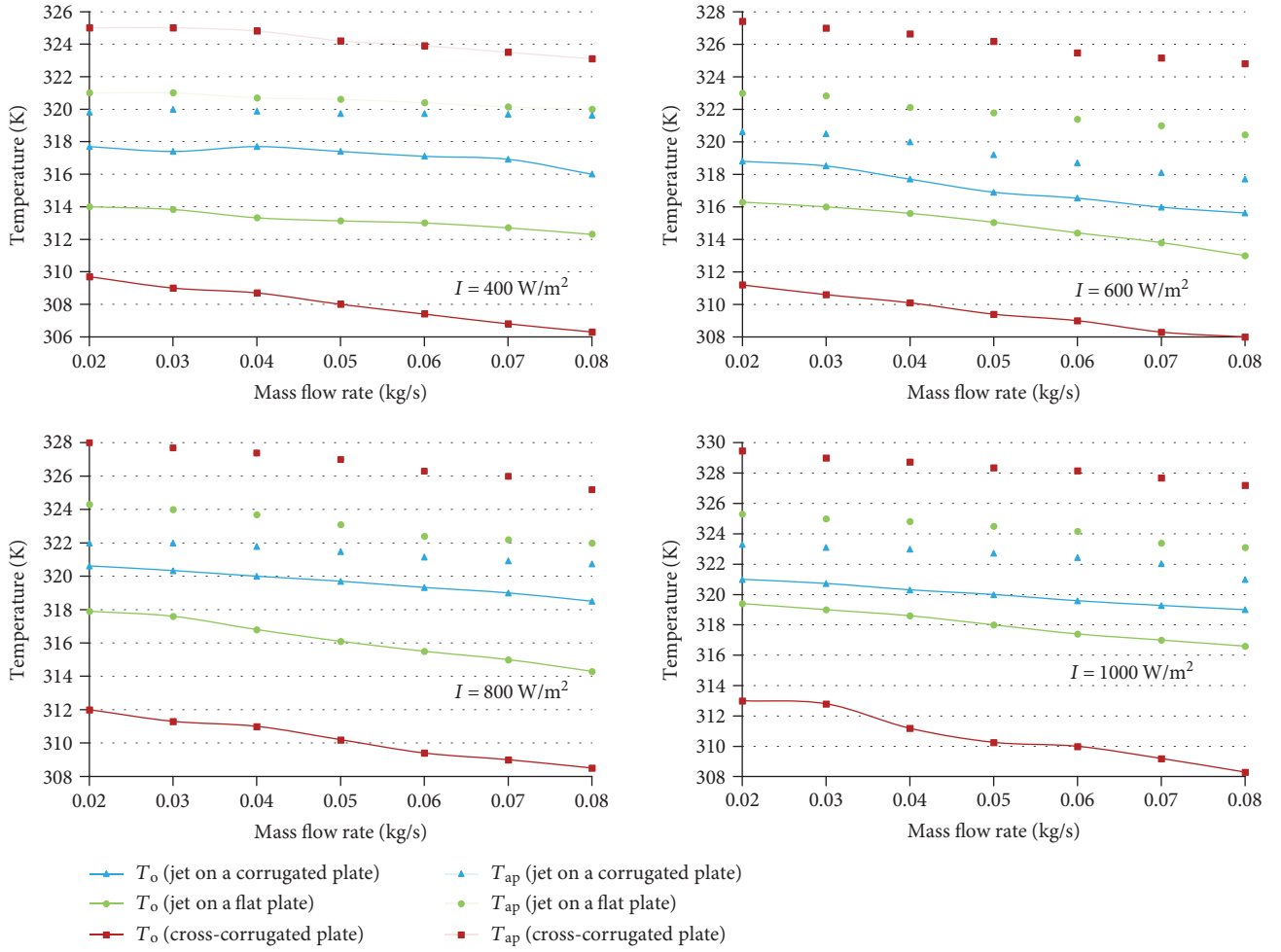
FIGURE 16: Absorber plate and outlet temperature of different collector designs versus mass flow rate for different solar radiation levels.
