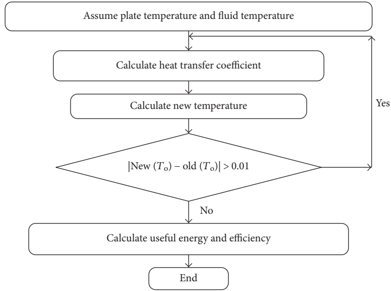
FIGURE 12: Block diagram of the calculation steps.
