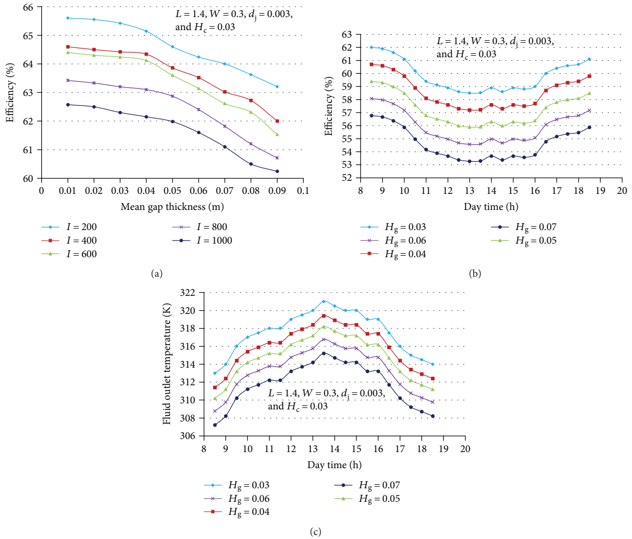
FIGURE 22: Prediction of the optimum mean gap thickness between the absorber plate and the jet plate ( H_g ) of the proposed solar air heater. (a) SAH efficiency versus H_g at different solar radiation levels. (b) Hourly SAH efficiency over daytime at different H_g . (c) Hourly air outlet temperature at different H_g .
