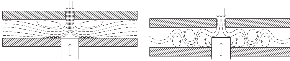
FIGURE 7: Characteristics of flow for a jet impinging on a flat surface and an actuating slab [35].
