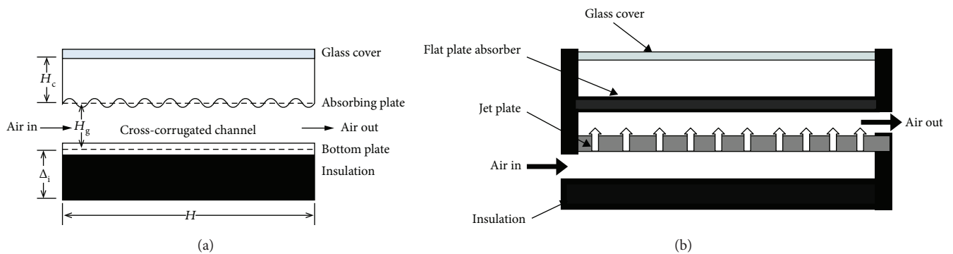
FIGURE 10: Schematic diagram of previous SAH designs (a) with a cross-corrugated absorber plate, Lin et al. [36] (b) with jet impingement on a flat absorber plate, Choudhury and Garg [37].
