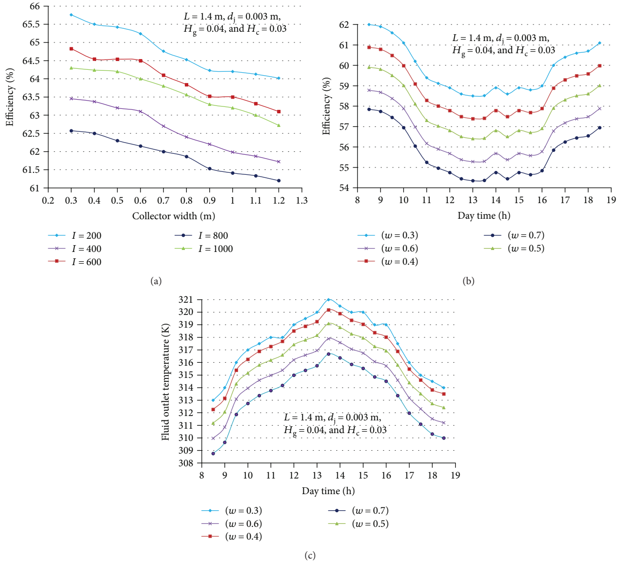
FIGURE 20: Prediction of the optimum width ( W ) of the proposed solar air heater. (a) SAH efficiency versus collector width at different solar radiation levels. (b) Hourly SAH efficiency over daytime at different collector widths. (c) Hourly air outlet temperature at different collector widths.
