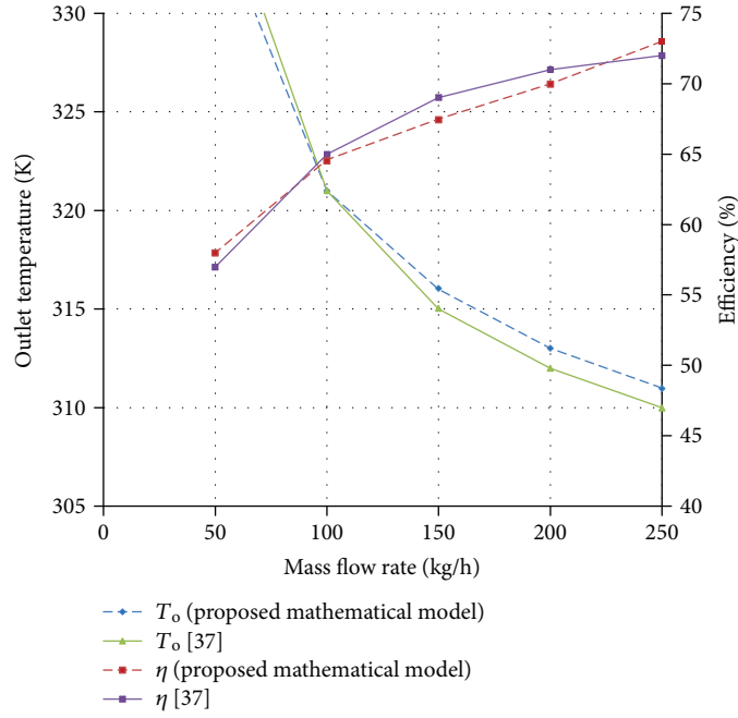
FIGURE 15: Predicted outlet temperature and efficiency of the SAH obtained from the proposed mathematical model and from reference work [37].
