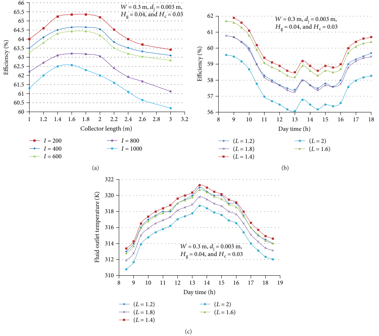
FIGURE 19: Prediction of the optimum length ( L ) of the proposed solar air heater. (a) SAH efficiency versus collector length at different solar radiation levels. (b) Hourly SAH efficiency over daytime at different collector lengths. (c) Hourly air outlet temperature at different collector lengths.
