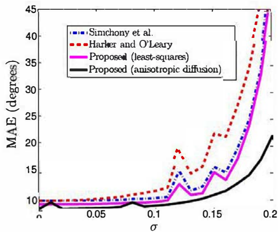
Fig. 11 Mean angular error (in degrees) as a function of the standard deviation \sigma \|I\|_{\infty} of the noise which was added to the photometric stereo images. The anisotropic diffusion approach always outperforms least squares. For the methods [26,53], the gradient field was filled with zeros outside the reconstruction domain, which adds even more bias
