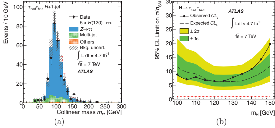
Fig. 1. – (a) Reconstructed m_{\tau\tau} of the selected events in the H \rightarrow \tau_{\text{had}}\tau_{\text{had}} channel. Expectations from the Higgs boson signal ( m_H = 120 \text{ GeV} ) and from backgrounds are given. (b) Observed (solid) and expected (dashed) 95% confidence level upper limits on the signal cross section times branching ratio for this channel, normalised to the SM expectation, as a function of the Higgs boson mass. Expected limits are given for the scenario with no signal. The bands around the dashed line indicate the expected statistical fluctuations of the limit.
