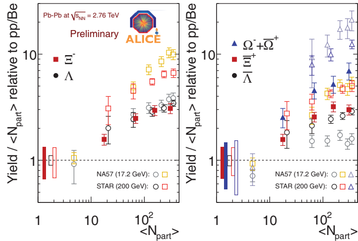
Fig. 2. – Enhancements in |y| < 0.5 as a function of the mean number of participants N_{\text{part}} measured by ALICE and compared to SPS and RHIC data. The bars on the dotted line indicate the systematic uncertainties on the pp reference.
