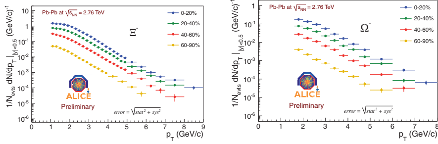
Fig. 1. – Transverse-momentum spectra of the \Xi^- and the \Omega^- in four centrality classes.
