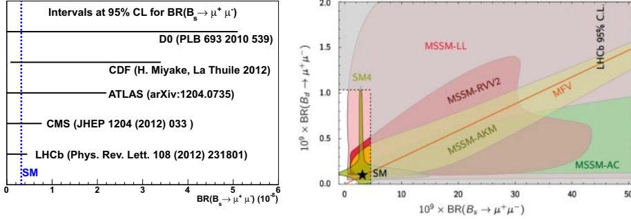
Fig. 1. – Left: Present limits on \mathcal{B}(B_s \rightarrow \mu^+\mu^-) at 95% CL set by the experiments D0 [9] CDF [10], ATLAS [11] CMS [12] and LHCb [13]. The SM prediction is indicated by the blue-dashed line. Right: Correlation for the branching fractions of the decays B_s \rightarrow \mu^+\mu^- and B_d \rightarrow \mu^+\mu^- for several models of physics beyond the SM. Details on the models can be found in [8]. The impact of the recent upper limits set by LHCb are shown as the shaded region. Reproduced from [14].
