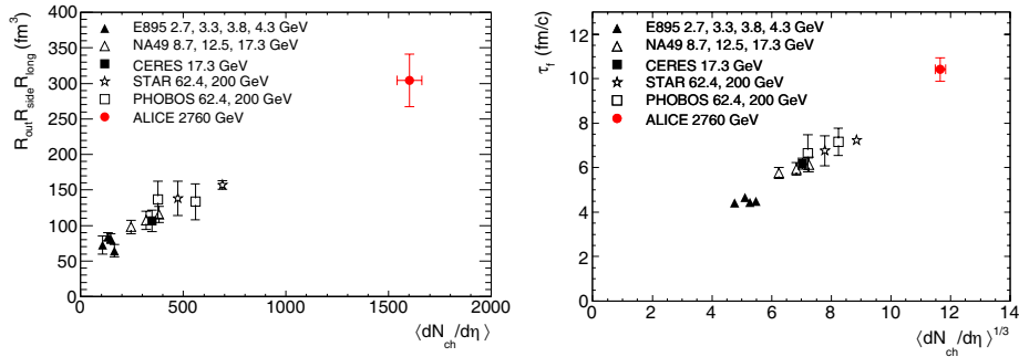
Fig. 4. – (Colour on-line) Femtoscopic measurements. Product of the three pion HBT radii (left) and decoupling time extracted from R_{long} (right). The ALICE results (red filled dots) are compared to those obtained for central gold and lead collisions at lower energies at the AGS, SPS, and RHIC. See [8] and references therein.
