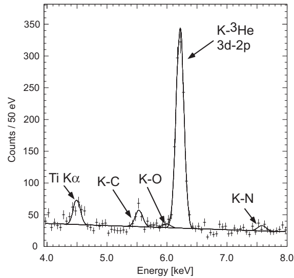
Fig. 2. – Energy spectrum of the kaonic ^3\text{He} X-rays in coincidence with the K^+K^- events. The kaonic ^3\text{He } 3d \rightarrow 2p transition is seen at 6.2 keV. Together with this peak, small other peaks are seen, which are the kaonic atom X-ray lines produced by the kaons stopping in the target window made of Kapton, and the \text{Ti } K\alpha line at 4.5 keV.
